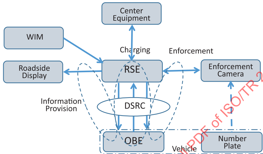
Figure 13 — Functional structure of toll-by-weight
