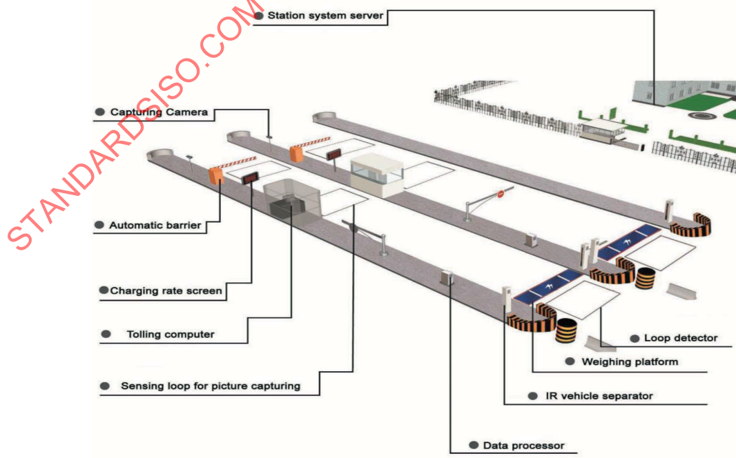
Figure A.7 — Overview of exit lane equipped with WIM (Source: Wanji technology in China)
