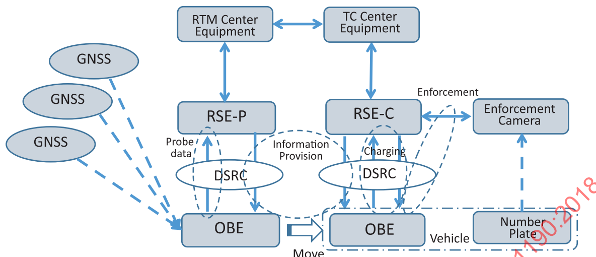
Figure 7 — Functional structure of probe data supported EFC
