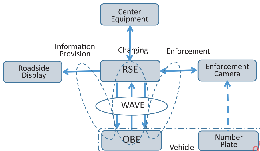
Figure 10 — Functional structure of WAVE based EFC
