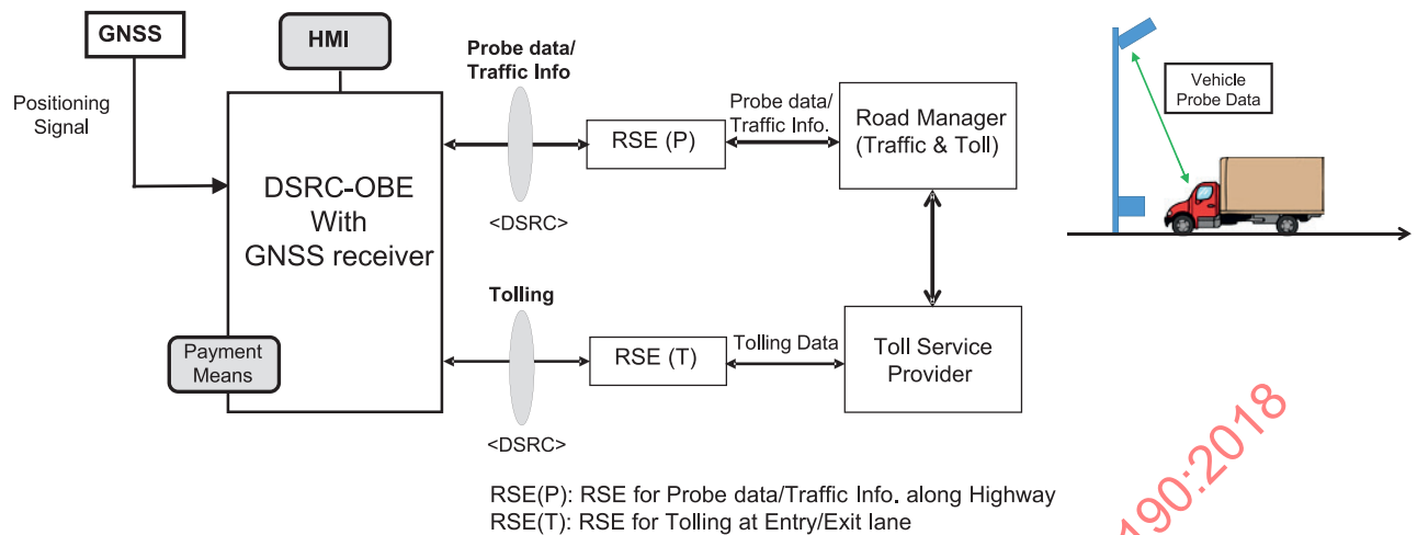
Figure A.2 — System configuration of smart route selection
