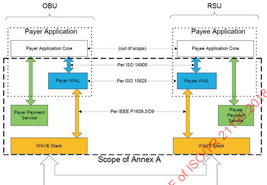
Figure 11 — EFC application on WAVE stack (Source: IEEE 1609.11)[5]
