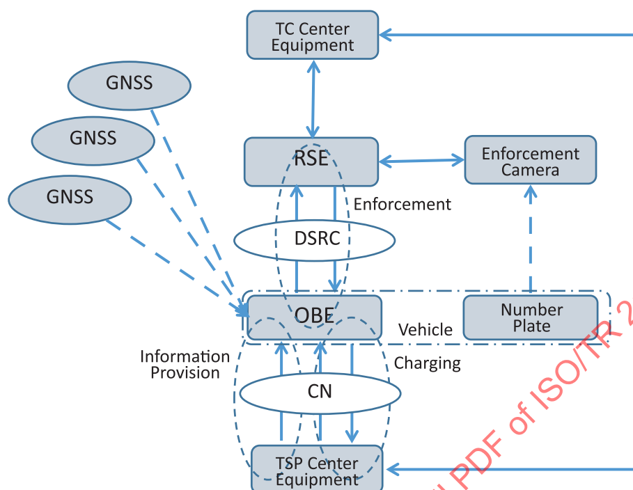
Figure 5 — Functional structure of autonomous systems
