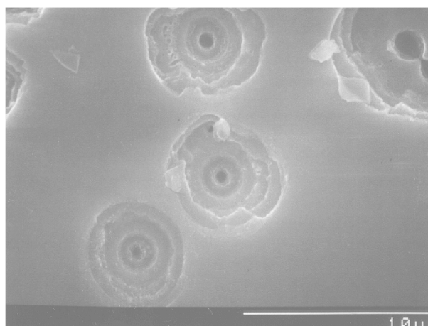
b) QWOT-stack HfO 2 /SiO 2 , Nd:YAG-Laser, \tau = 14 ns, defect-induced damage
