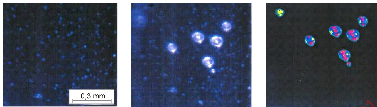
a) Example of the evaluation of microscopic images recorded before irradiation (TEA-CO 2 -Laser) of sample surface
