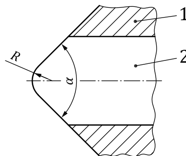
Figure 19 — Set-up of the device for the scratch test with conical stylus 3
