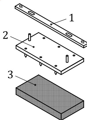
Figure 45 — Set-up of the device for the scrub test with non-woven web 1
