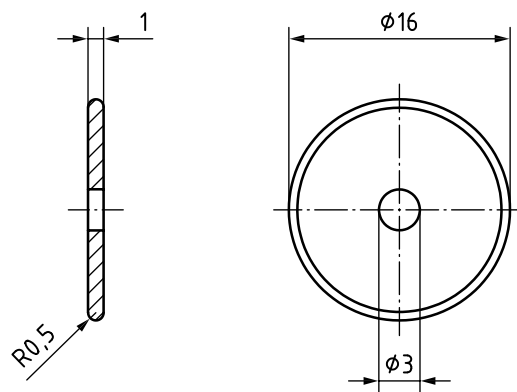
Figure 30 — Dimensions of the test disc
