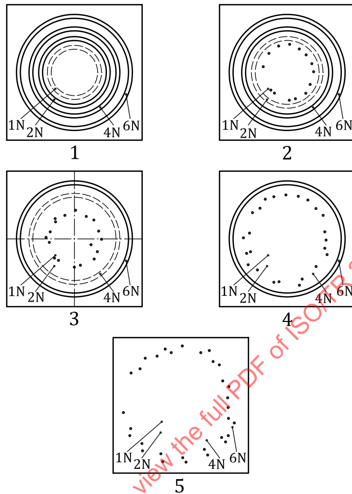
Figure 21 — Reference images for degree 1 to degree 5
