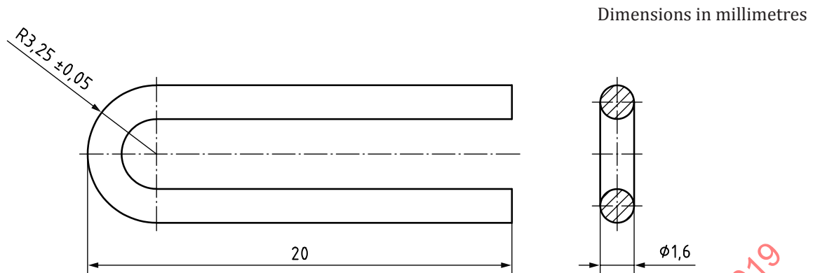
Figure 32 — U-shaped stylus
