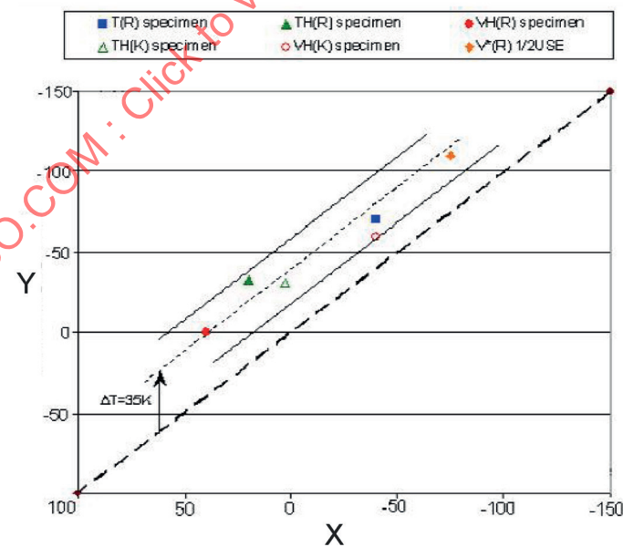
Figure A.29 — Ductile-Brittle-Temperature-Transition — Comparison of T_{1/2} (USE) to FATT of sub-size specimens (SUS)
