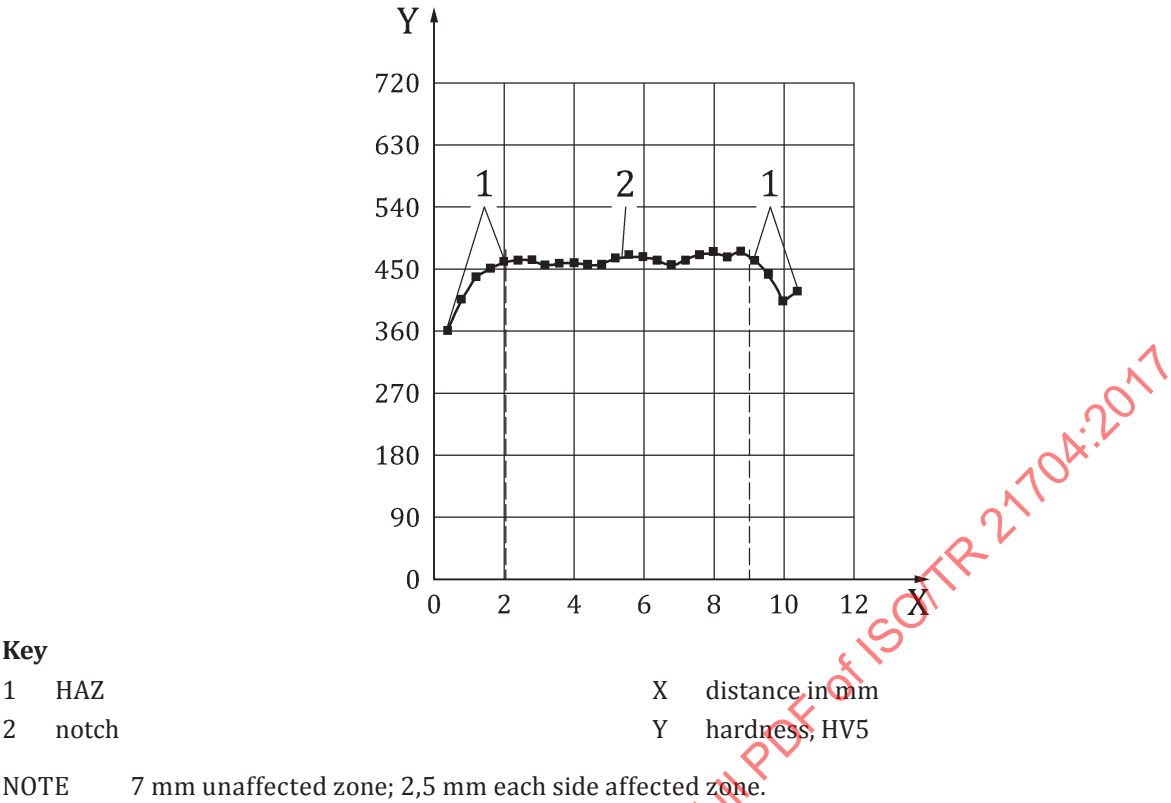
Figure A.32 — Laser welded-on — Hardness measurement
