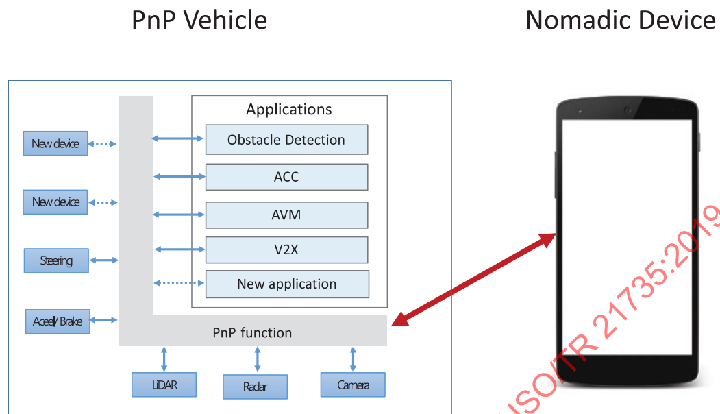
Figure 1 — Framework architecture for in-vehicle PnP
