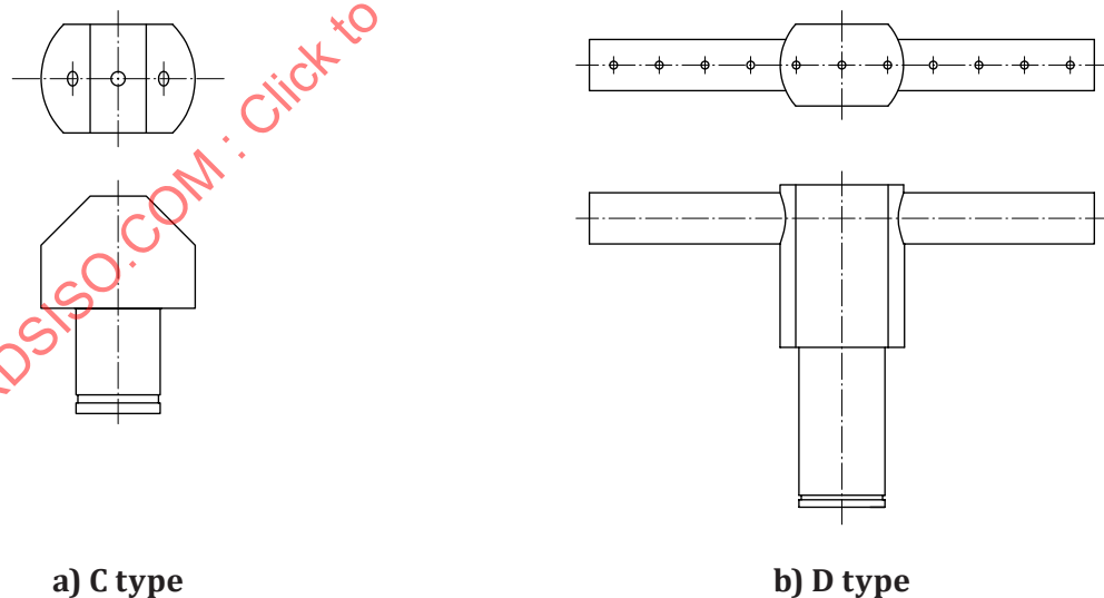
Figure 7 — Nozzle types for tilting pad journal bearing
