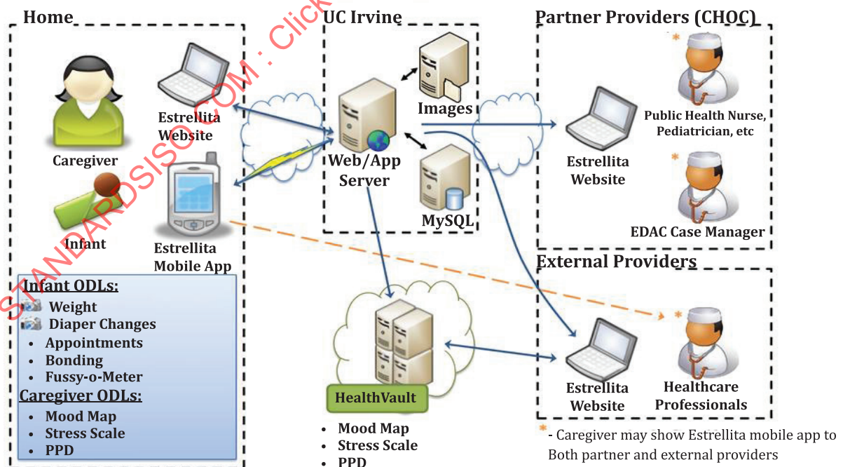
Figure 2 — Estrellita™ 2) application technical architecture diagram [6]
