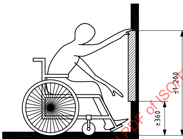
Figure 23 — Unobstructed forward reach (full mobility of the upper body and arms)
