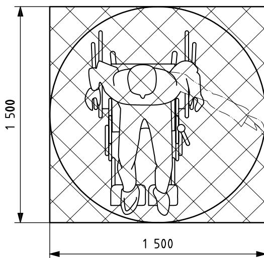
Figure 20 — Manoeuvring clearance
