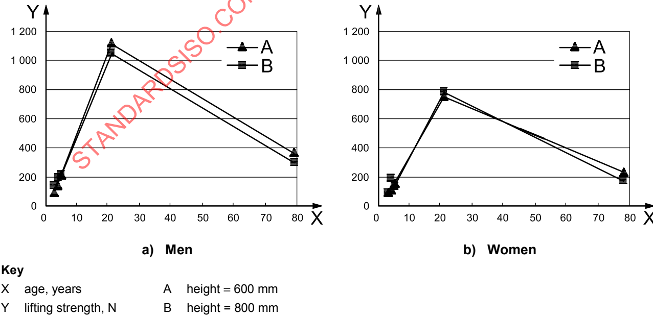
Figure 64 — Lifting strength data for healthy Japanese men and women during childhood, youth and old age
