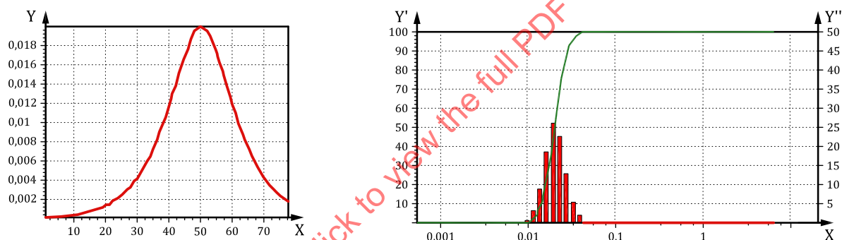
a) Mean particle diameter 20 nm
