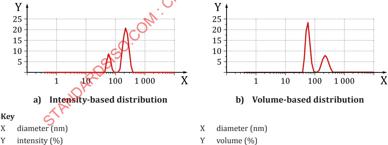
Figure 6 — Intensity based and volume-based distribution of a 2:1 volume mixture of particles of 60 nm and 220 nm diameter polystyrene latex particles
