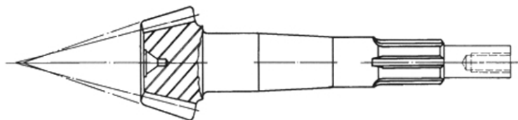
Figure 8 — Shank-type pinion with tapped hole
