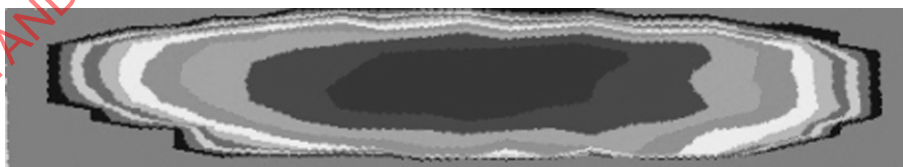
Figure 21 — Calculated loaded contact pattern
