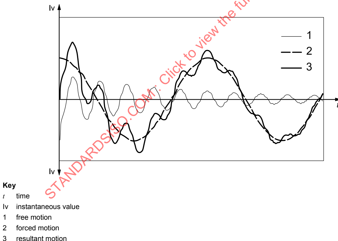
Figure 12 — Starting transient for forced vibrations
