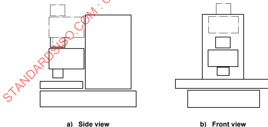
Figure 17 — Two views of a basic machine tool showing two carrier positions
