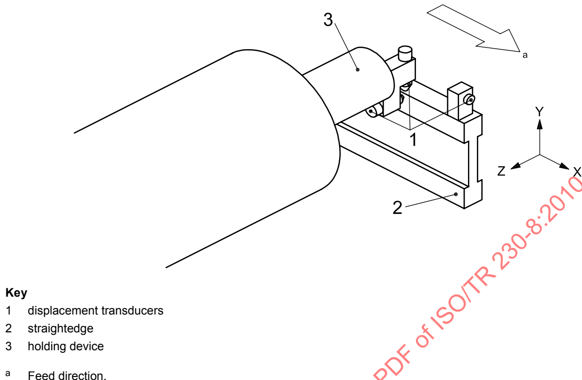
Figure 27 — Example of set-up using a straightedge
