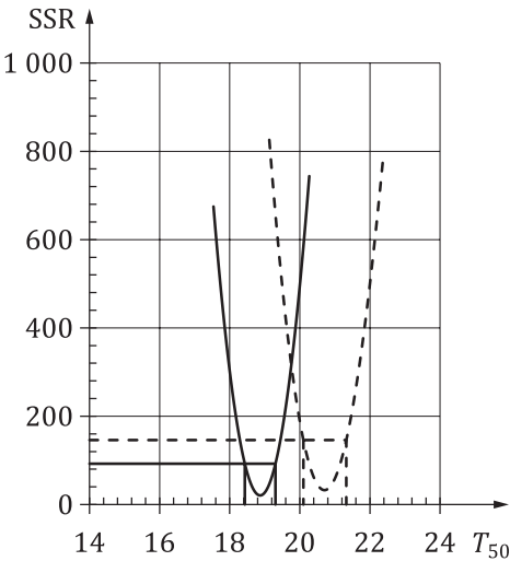
Figure 12 — 95 % confidential intervals of T_{50} in the UFB section and the control section of high-quality barley seeds (sample No. 2 in Table 1)
