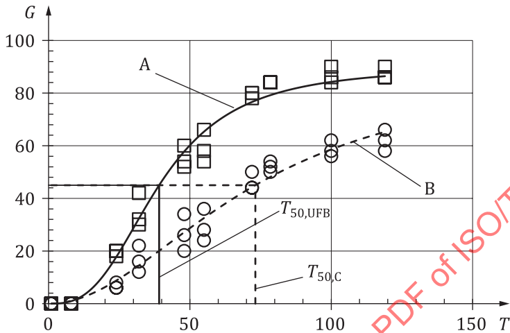
Figure 4 — Promoting the germination of low-quality barley seeds by UFB (sample No. 5 in Table 1)
