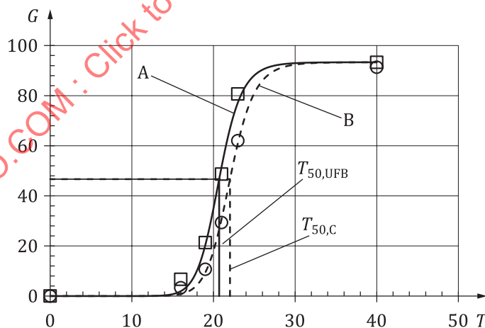
Figure 19 — Promoting the germination of high-quality barley seeds by UFB (sample No. 9 in Table 1)
