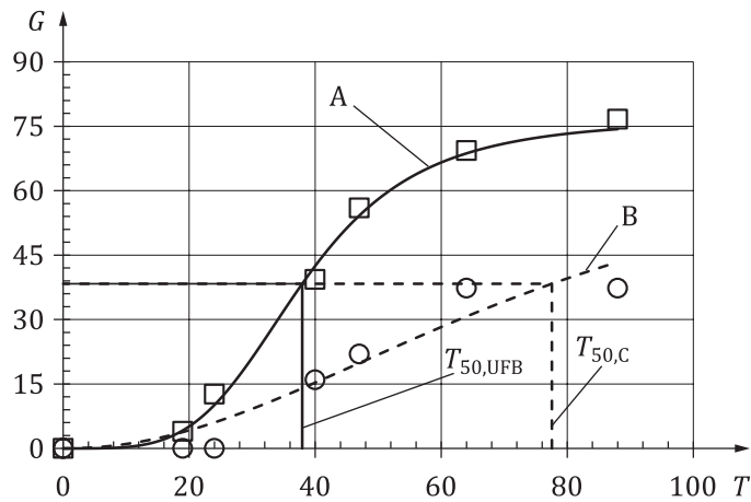
Figure 28 — Promoting the germination of low-quality barley seeds by UFB (sample No. 10 in Table 1 )
