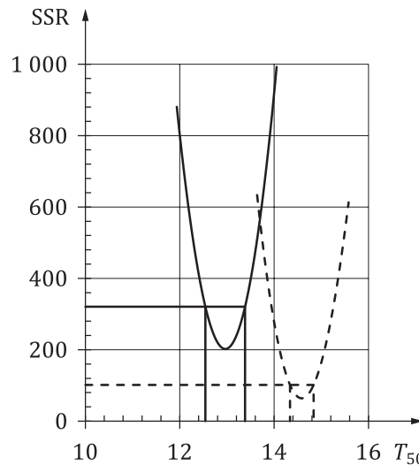
Figure 18 — 95 % confidential intervals of T_{50} in the UFB section and the control section of high-quality barley seeds (sample No. 4 in Table 1)
