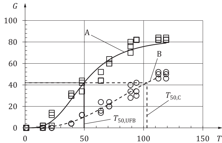
Figure 22 — Promoting the germination of low-quality barley seeds by UFB (sample No. 6 in Table 1 )
