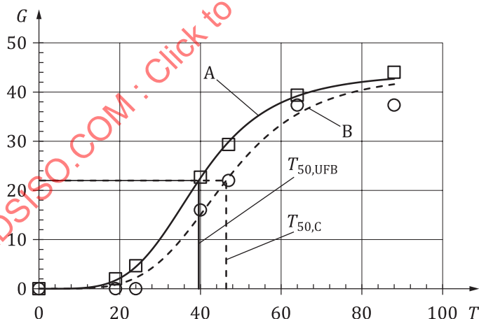
Figure 25 — Promoting the germination of low-quality barley seeds by UFB (sample No. 7 in Table 1)
