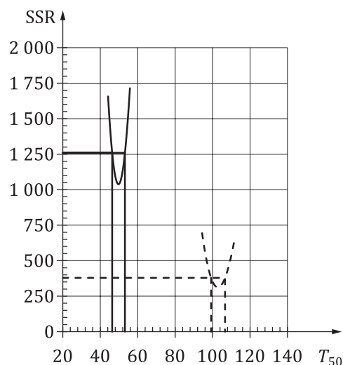
Figure 24 — 95 % confidential intervals of T_{50} in the UFB section and the control section of high-quality barley seeds (sample No. 6 in Table 1)
