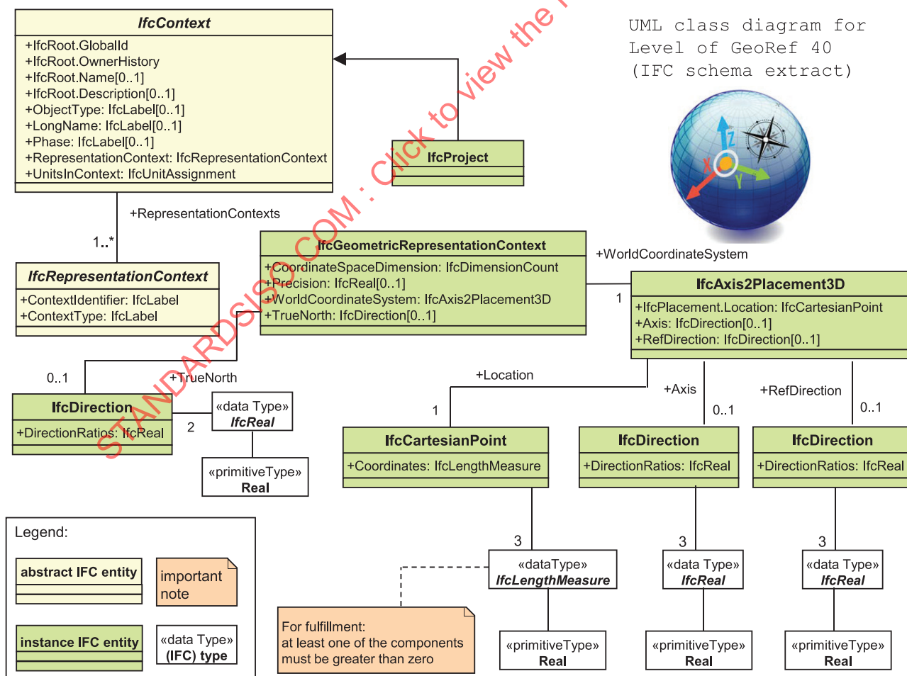
Figure C.5 — IFC entities to specify the geometric representation context of a project (LoGeoRef 40)
