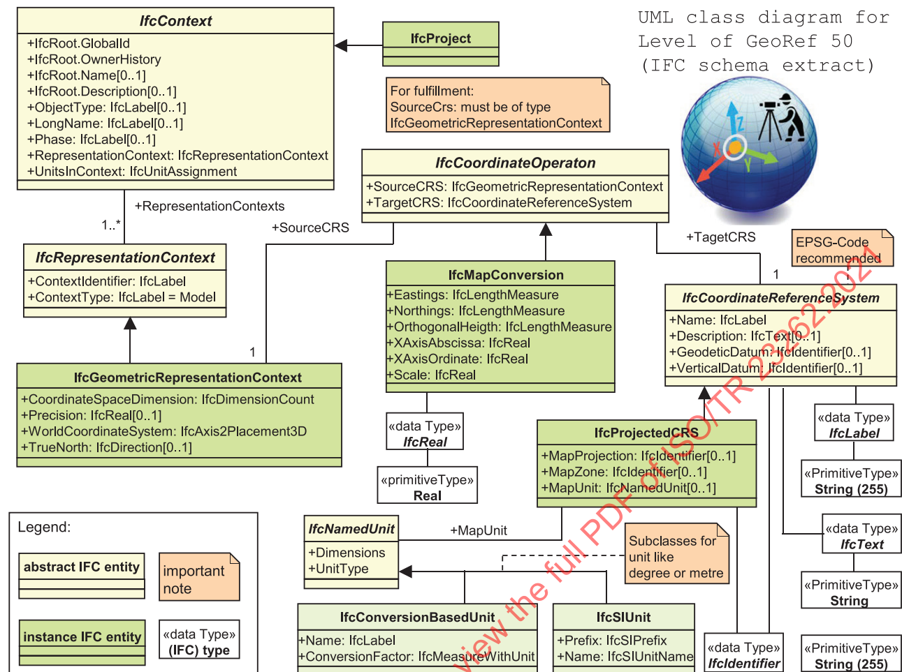
Figure C.6 — IFC entities to specify georeferencing with metadata in IFC4 (LoGeoRef 50)
