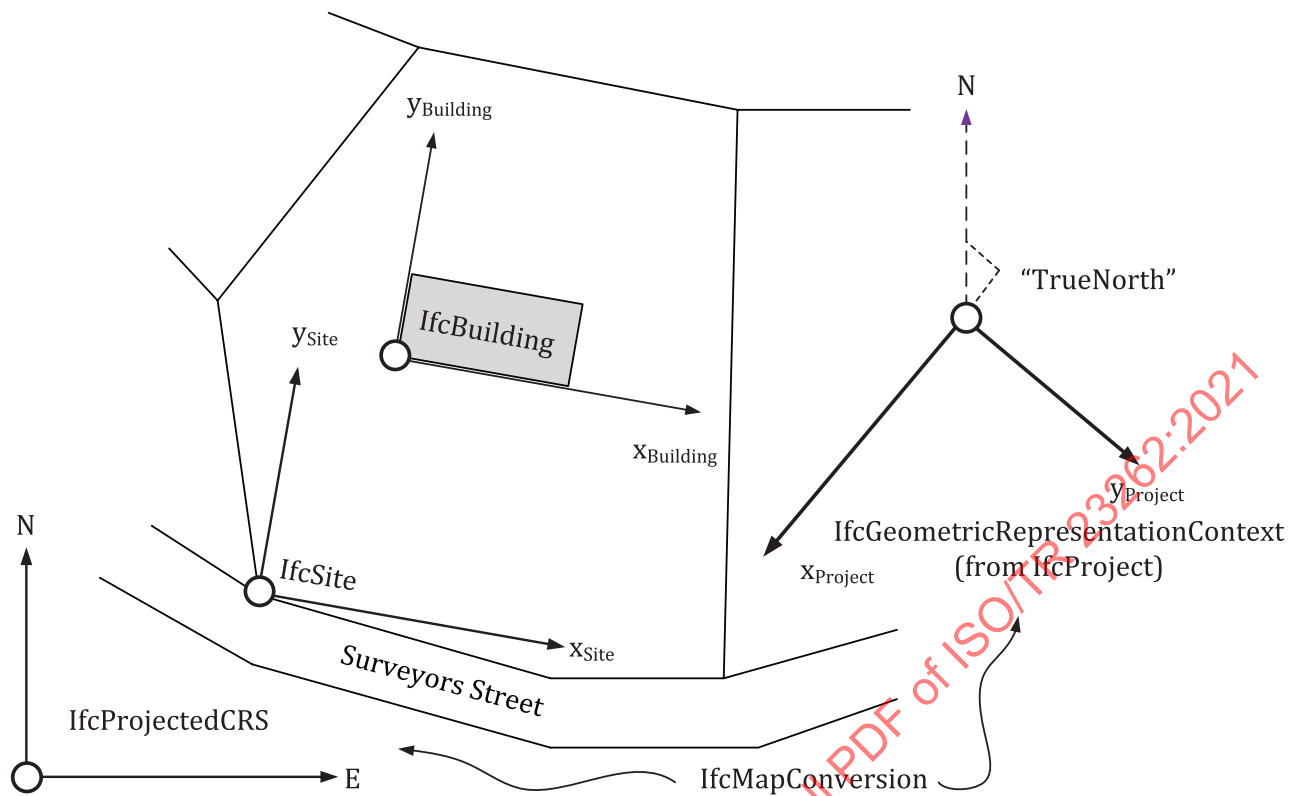
Figure C.1 — Cascading relative CRS for a BIM Project (for a BIM building model)
