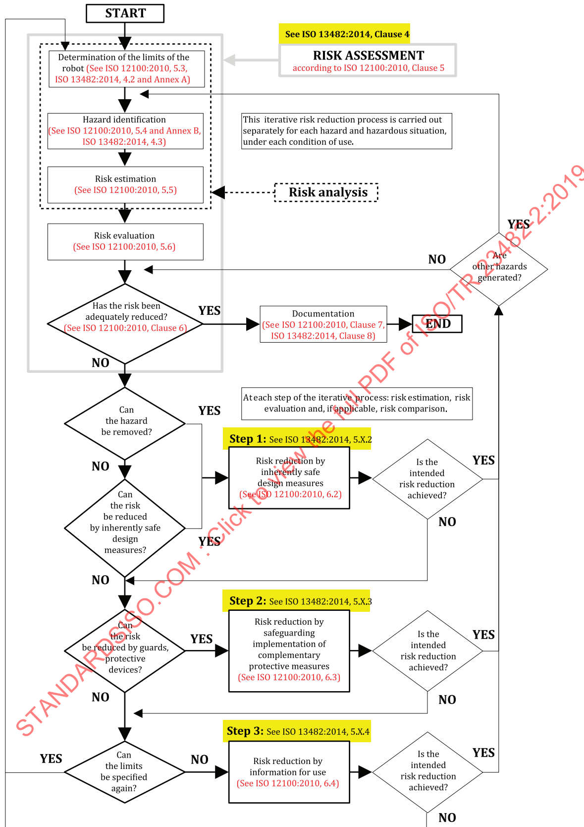
Figure 2 — Schematic representation of risk reduction process with extended information for users of ISO 13482
