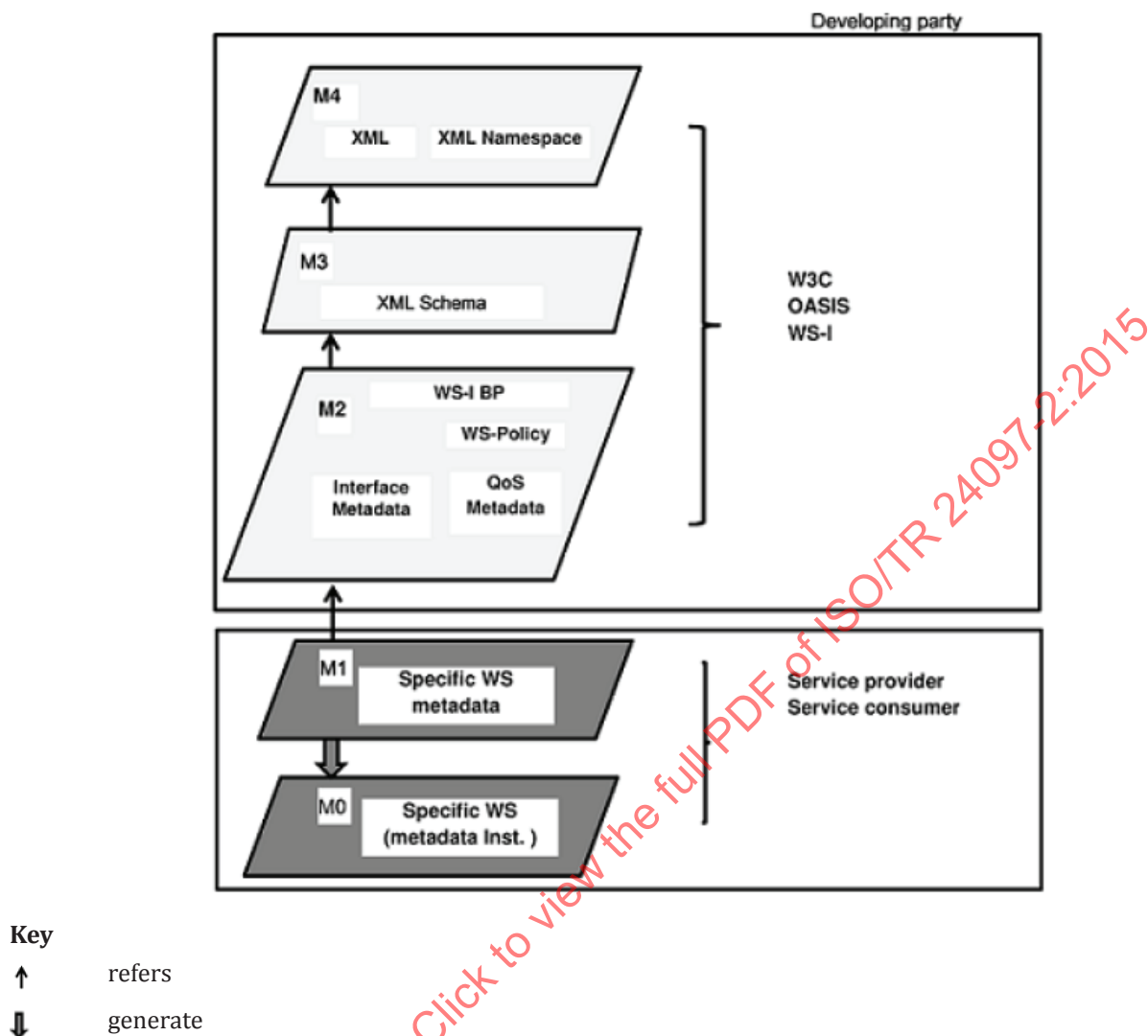
Figure 4 — Specific WS metadata, specific WS, and XML standards relationship
