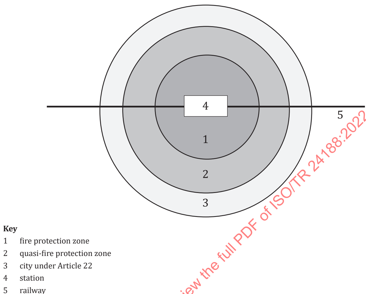
Figure 2 — Zoning concept according to BSL of Japan (from Reference [25])
