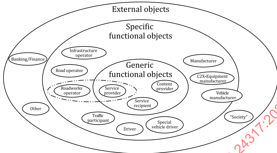
Figure 2 — Relation between generic and specific operation (ISO 17427-1:2018)
