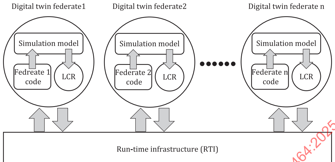
Figure B.2 — Digital twin federation based on high-level architecture (HLA)
