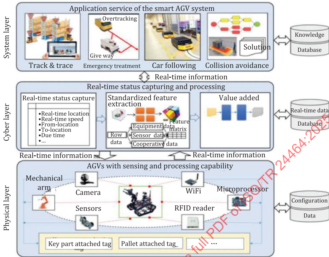
Figure C.6 — Instance of data management system [14]
