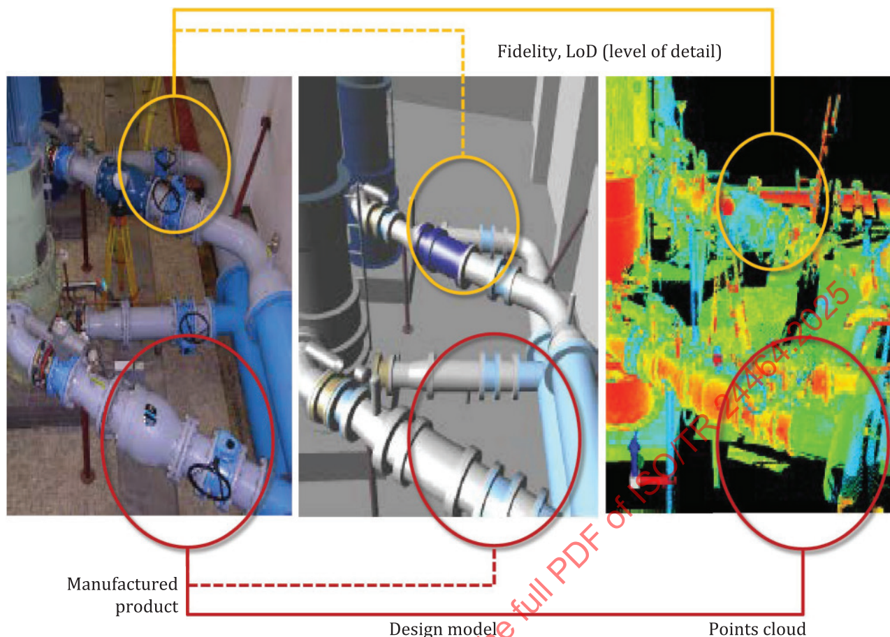
Figure 14 — Laser-scanned point cloud for verifying design model against manufactured product [35]
