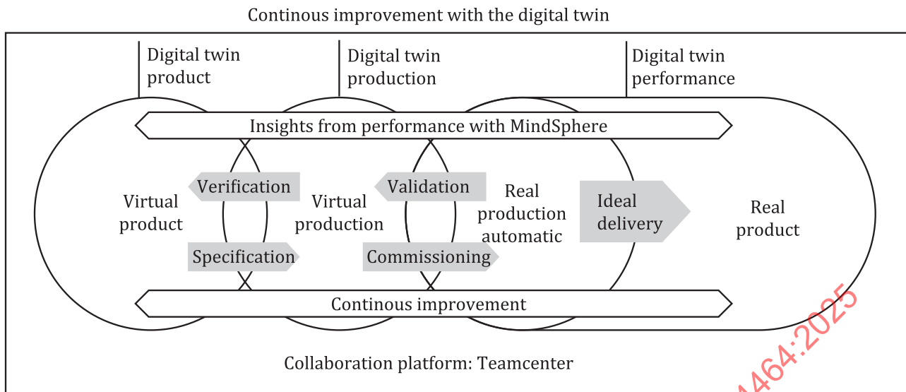
Figure 9 — Life cycle model of DTw
