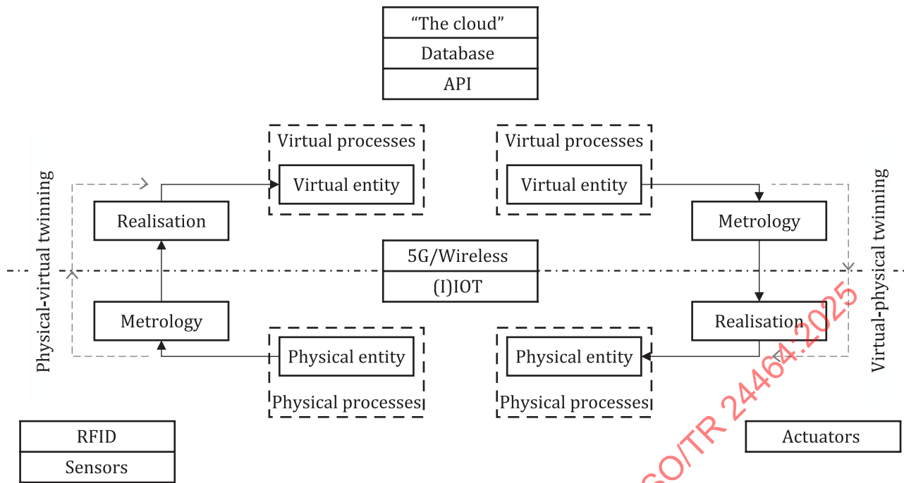
Figure C.3 — Technology mapped to the twinning cycle
