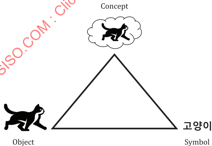
Figure 13 — Semiotic triangle
