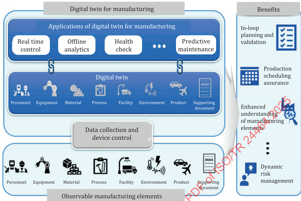
Figure C.7 — Concept of DTw for manufacturing [11]
