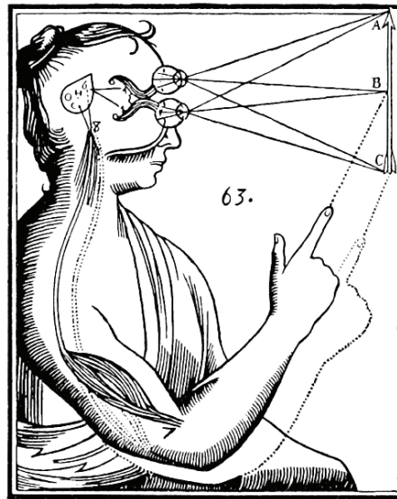
Figure 12 — Mind-body problem [41]
