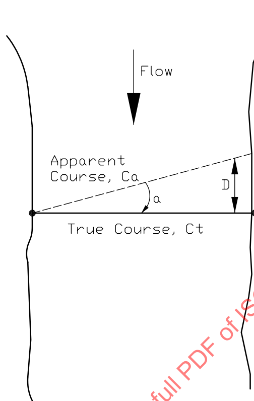
Figure 12 — Azimuth method
