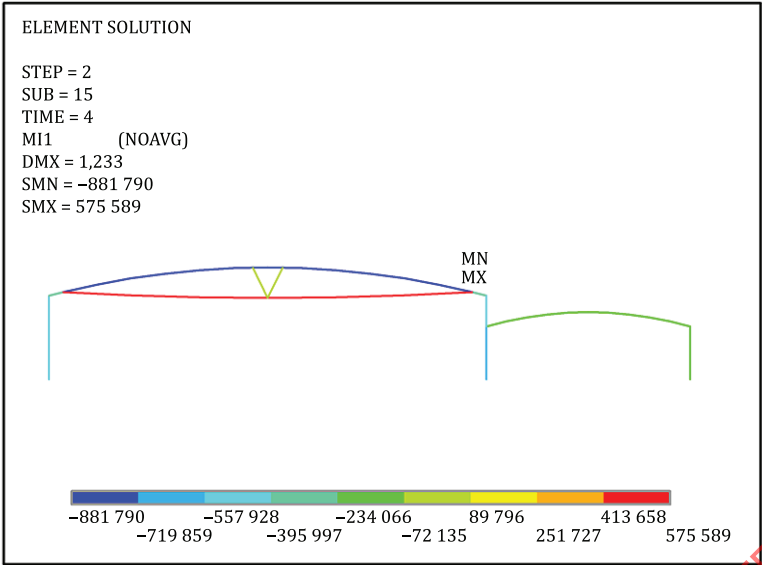
Figure 23 — Axial force of the frame (N)
