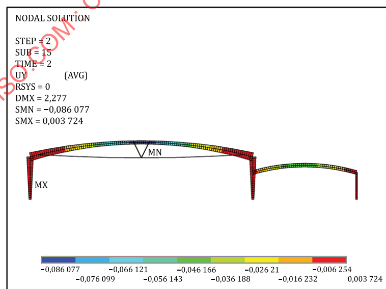
Figure 15 — Vertical calculated displacements of the steel frame (m)
