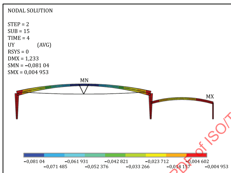
Figure 16 — Vertical deformation calculation (m)
