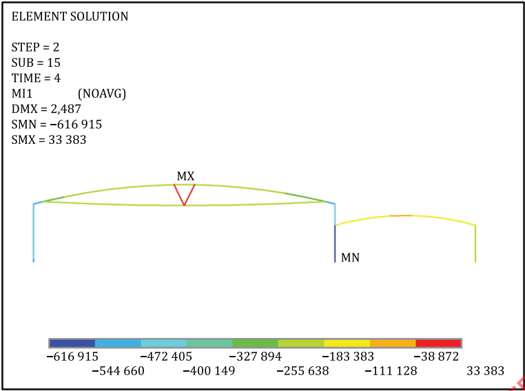
Figure 19 — Axial force of the frame (N)
