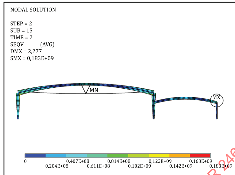
Figure 17 — Maximum von Mises stress (Pa)
