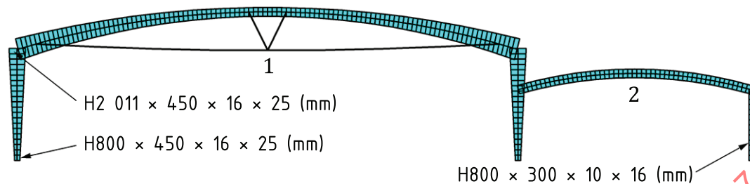
Figure 14 — Computational model of a single steel frame
