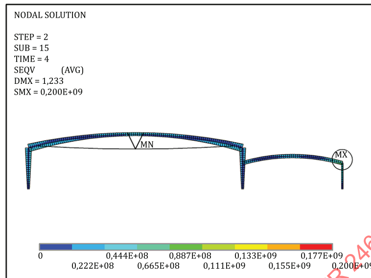
Figure 21 — Maximum von Mises stress (Pa)
