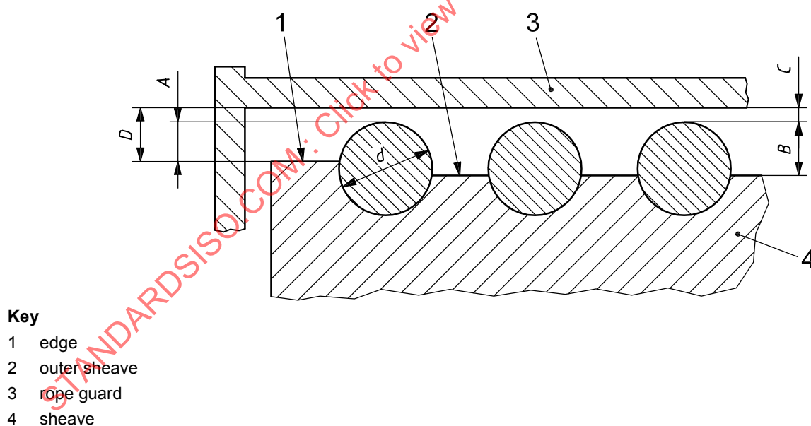
Figure A.5 — Installation standard of rope guard
