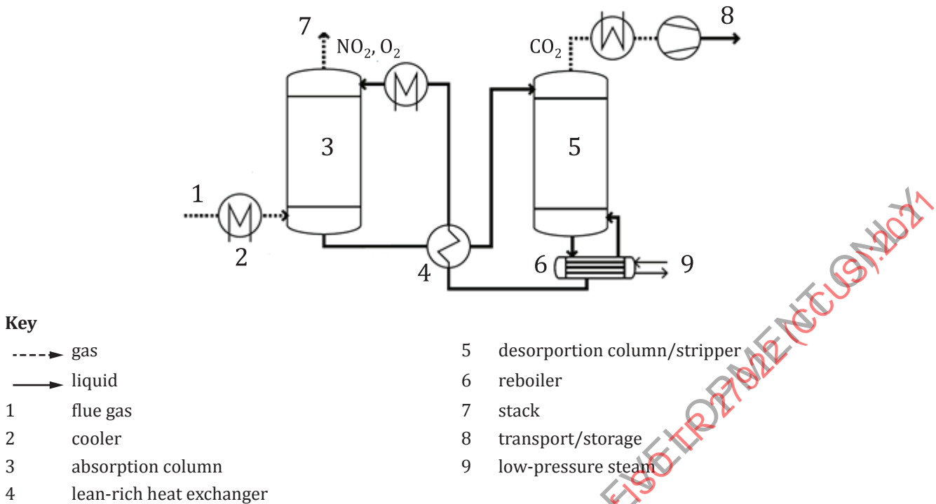
Figure 3 — Schematic representation of absorptive CO 2 capture [6]
