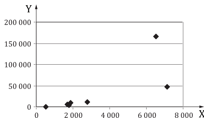
Figure 24 — Relationship between sampling variance and average
