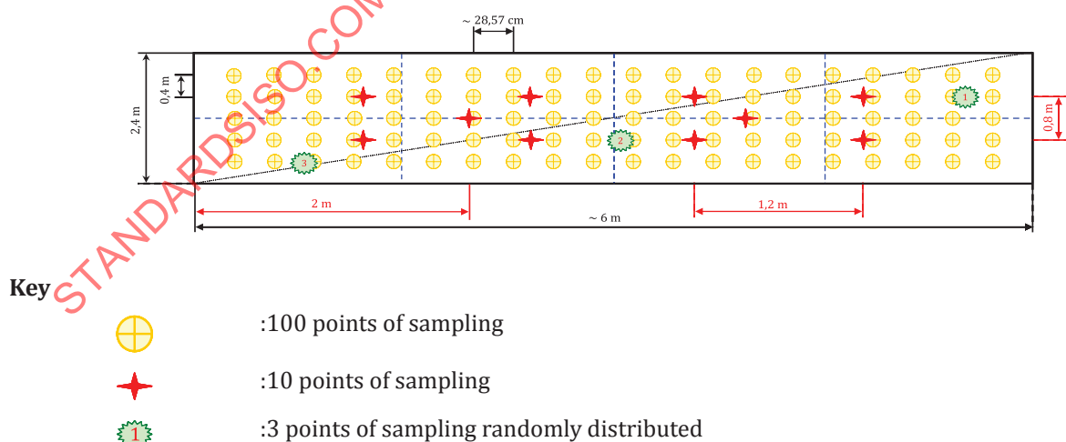
Figure 6 — Example of sampling from lorries
