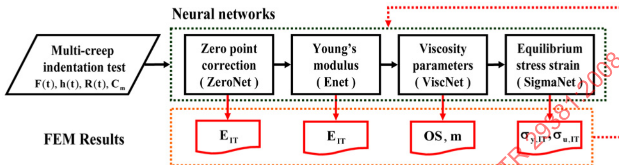
Figure 15 — Computational simulations
