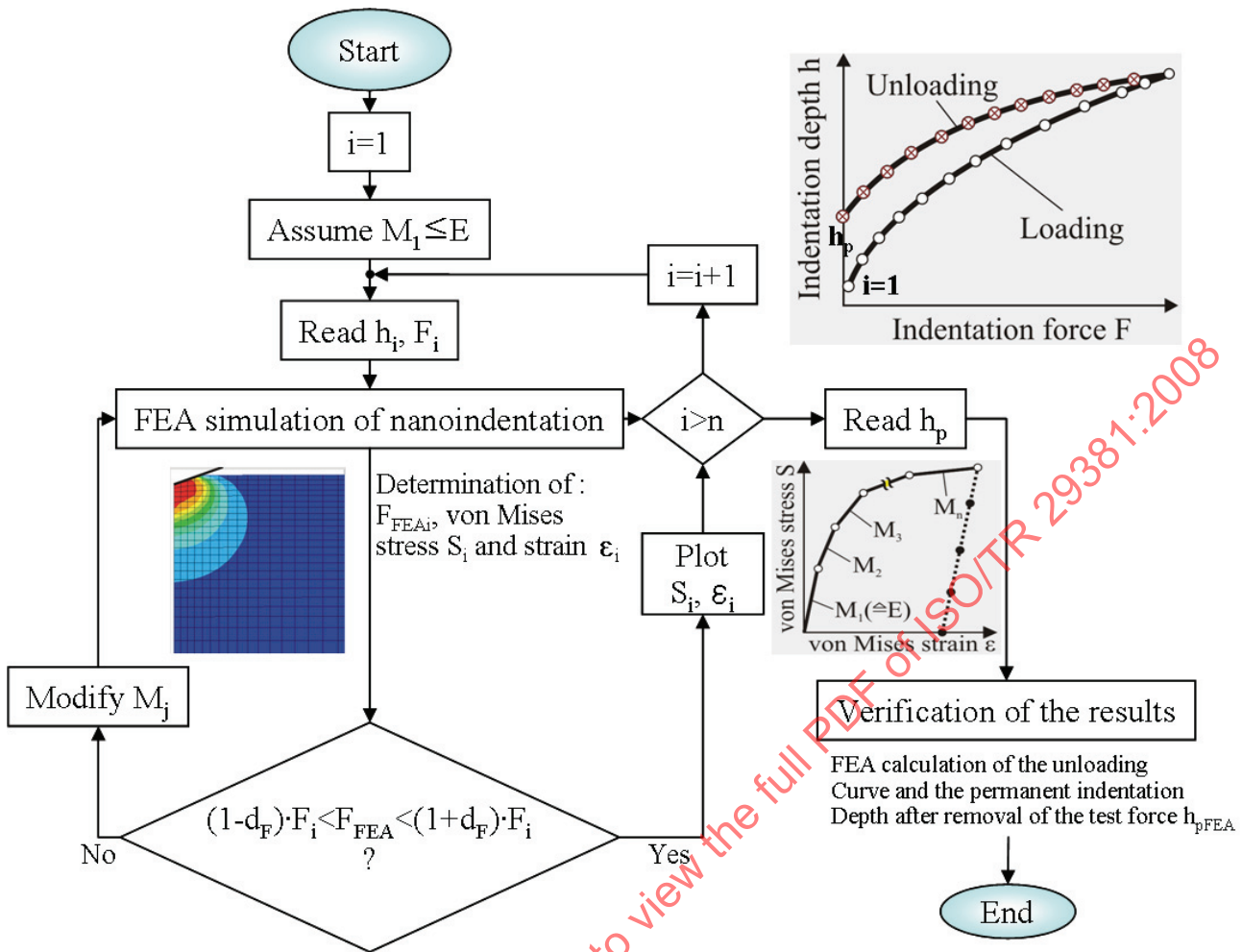
Figure 11 — Computational simulations
