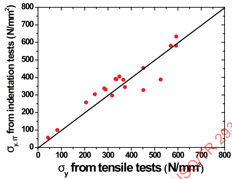
a) Yield strength
