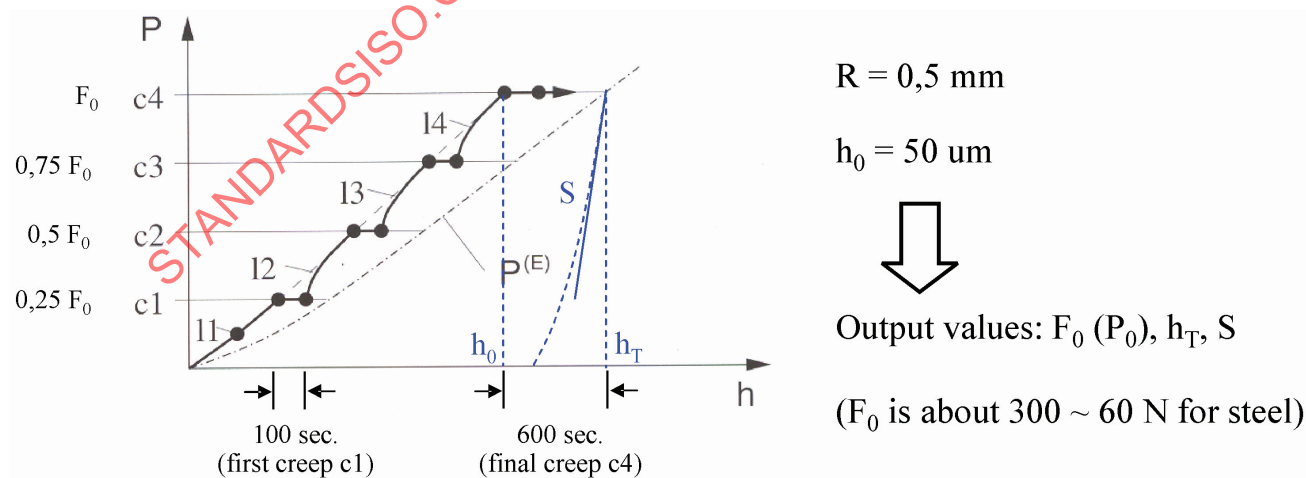
Figure 16 — Example of force-depth curve
