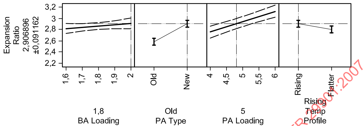
Figure D.4 — Expansion ratio prediction
