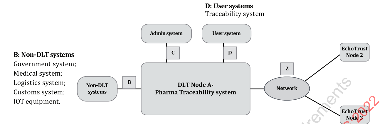
Figure 82 — Data flow analysis: Franchised pharma supply chain management (China)
