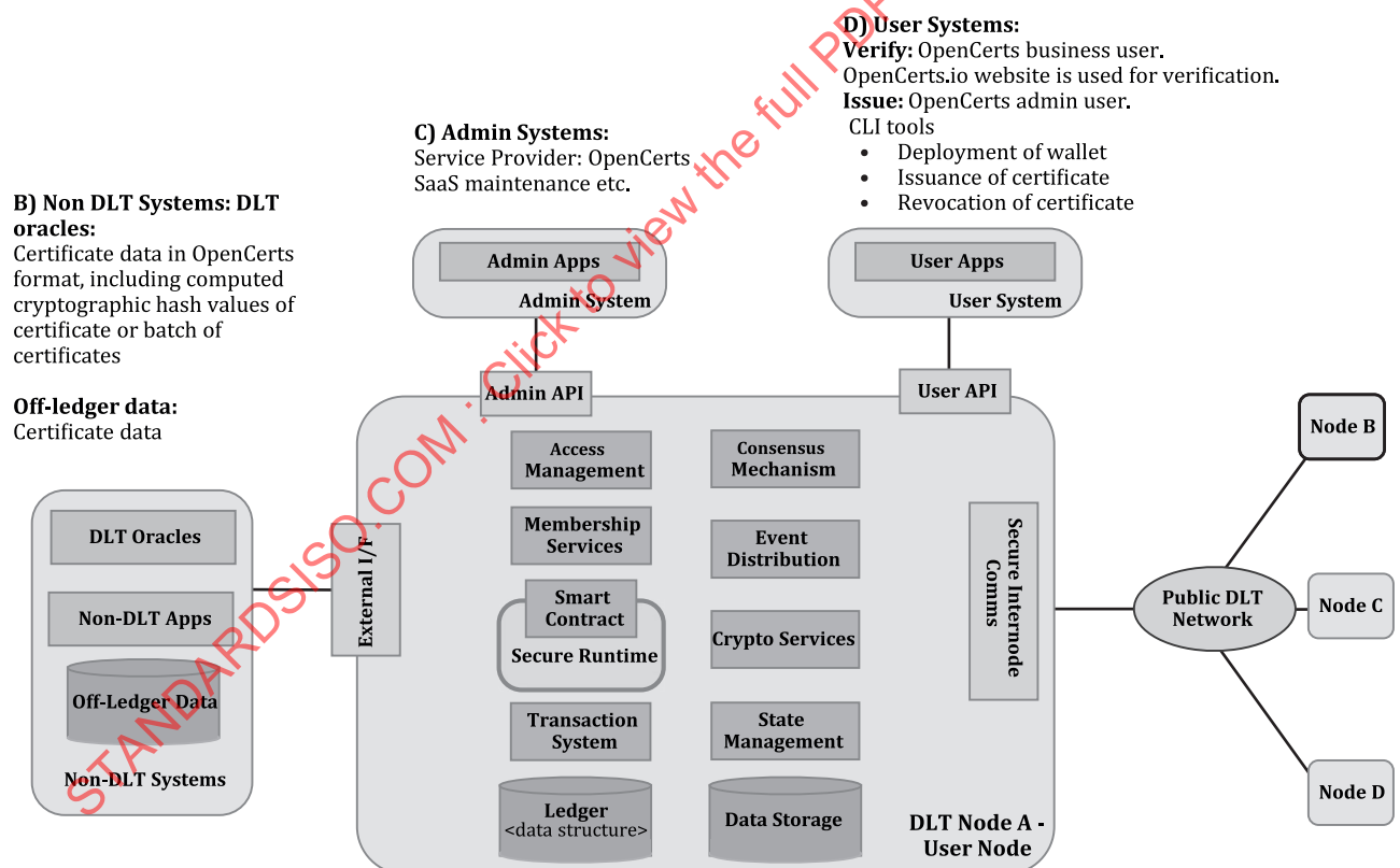
Figure 30 — System view architecture: Education Certificates Provenance (Singapore)
