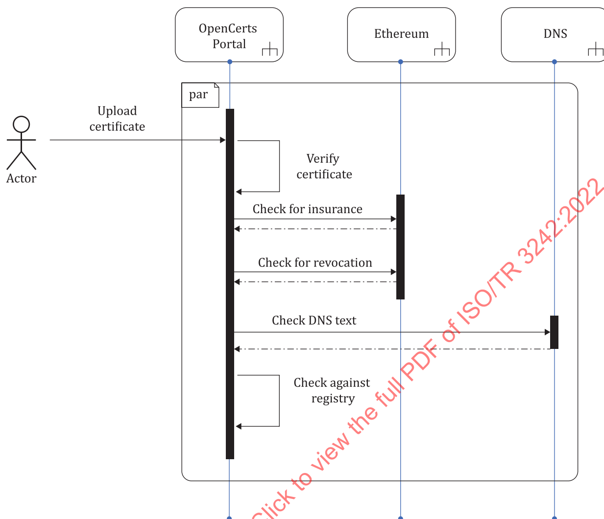
Figure 34 — Sequence diagram: Education certificates provenance (Singapore) – Verify Certificate
