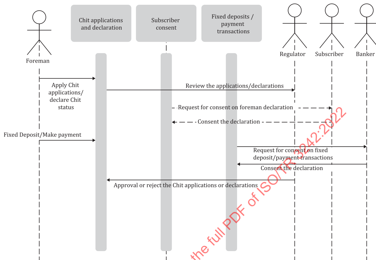
Figure 57 — Sequence Diagram: Organised Chit Funds (India)
