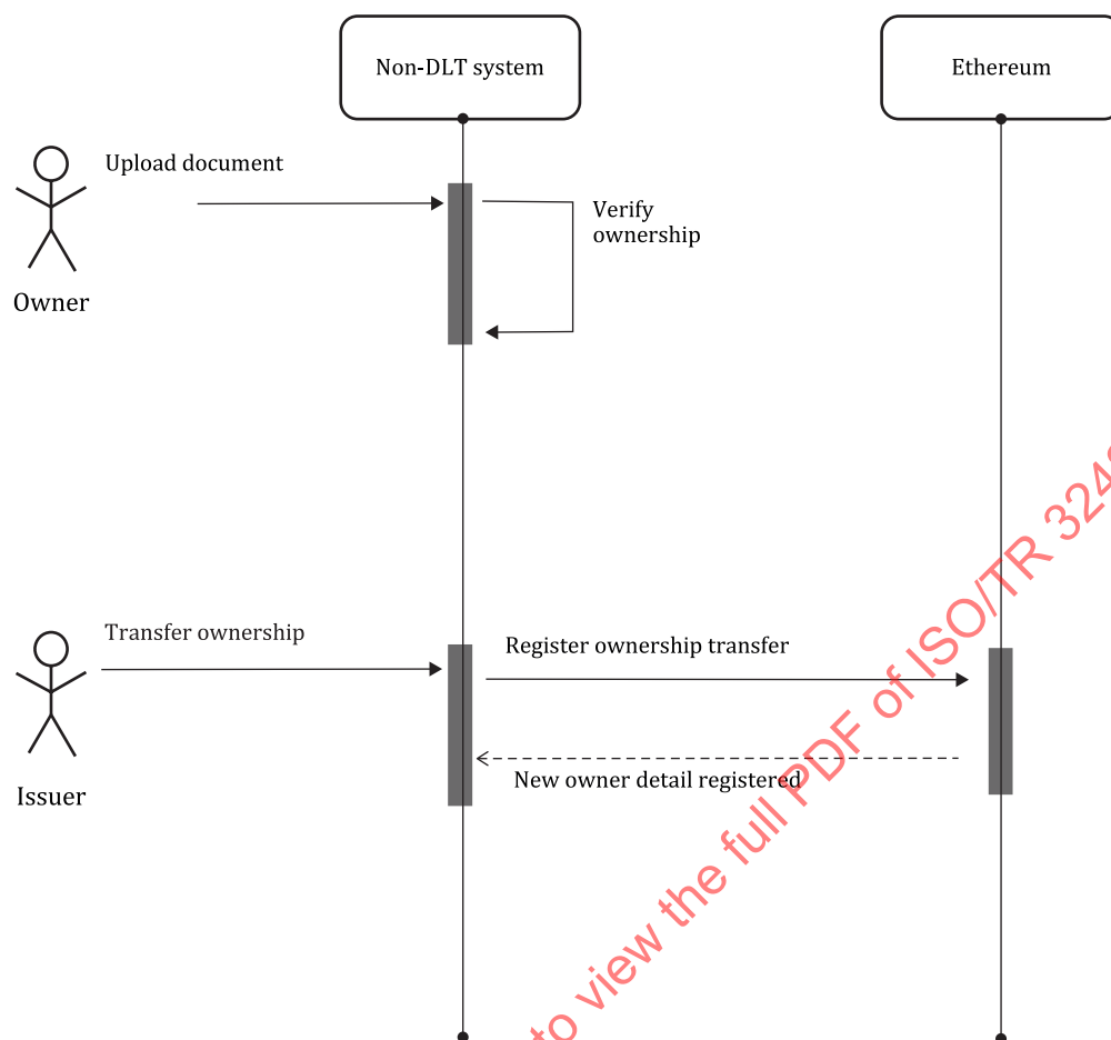
Figure 75 — Sequence diagram: International trade transparency (Singapore) -Transfer ownership of Bill of Lading
