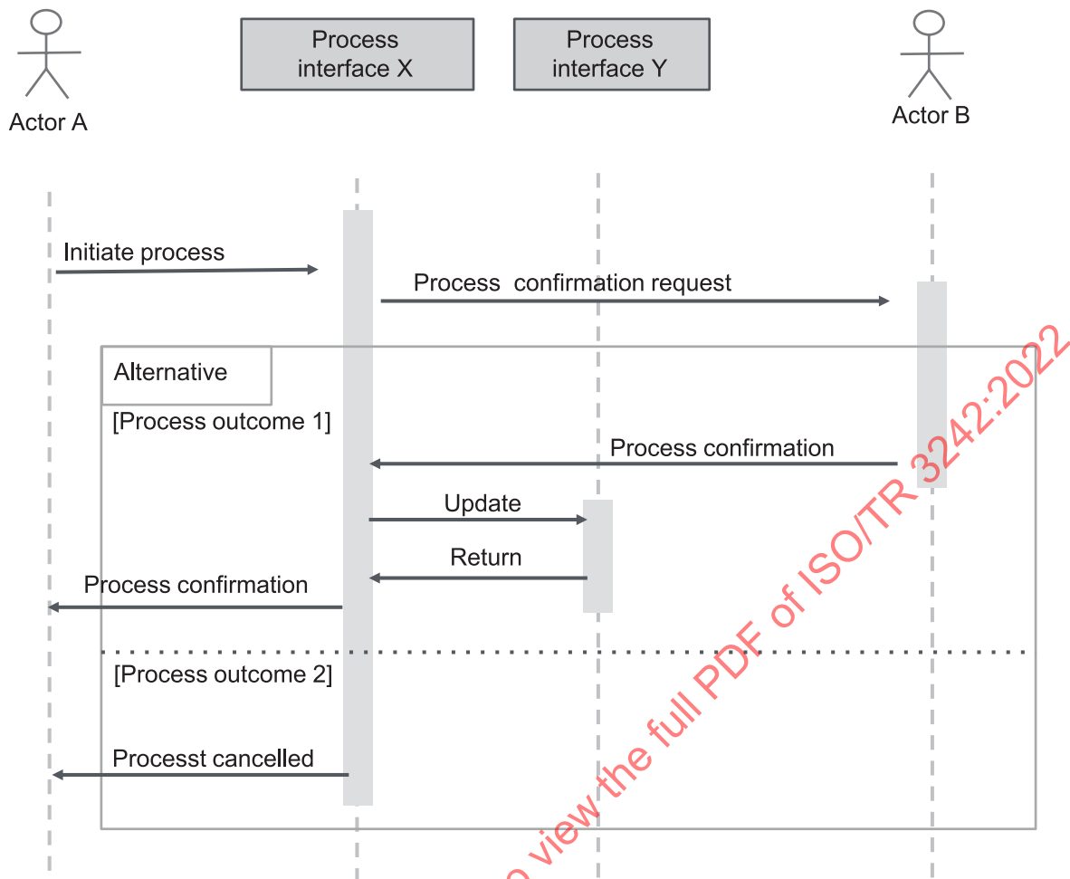
Figure 6 — Example sequence diagram
