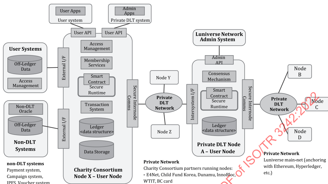
Figure 67 — Systems view architecture: Decentralised Charity Platform (the Republic of Korea)
