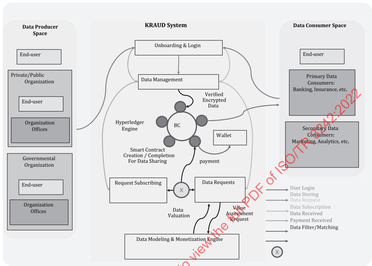
Figure 43 — Interaction diagram: SSI (Cyprus)
