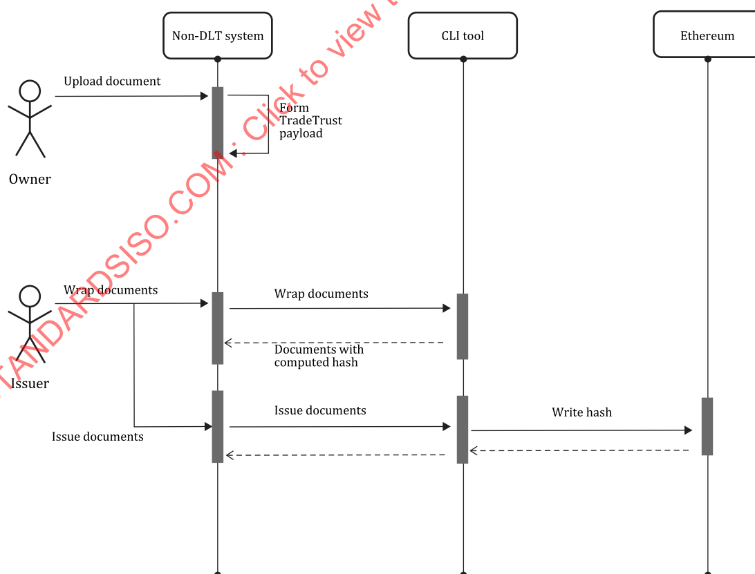
Figure 74 — Sequence diagram: International trade transparency (Singapore) - Issue Bill of Lading
