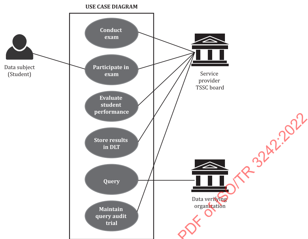
Figure 27 — Use case diagram: SRMS (India)
