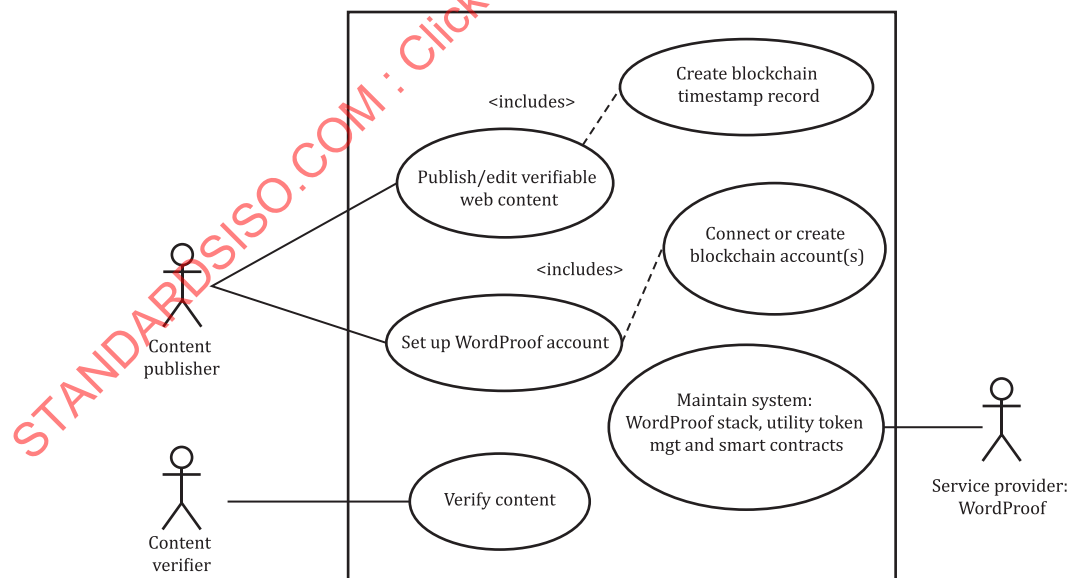
Figure 37 — Use case diagram: Content timestamp verification (Netherlands)
