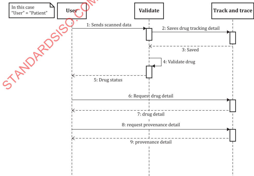
Figure 89 — Sequence diagram: Anti-counterfeit solution for pharma industry (India)
