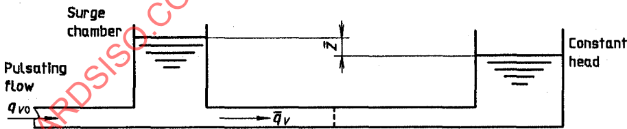
Figure 2 — Surge chamber
