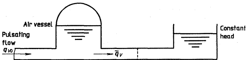
Figure 3 — Air vessel
