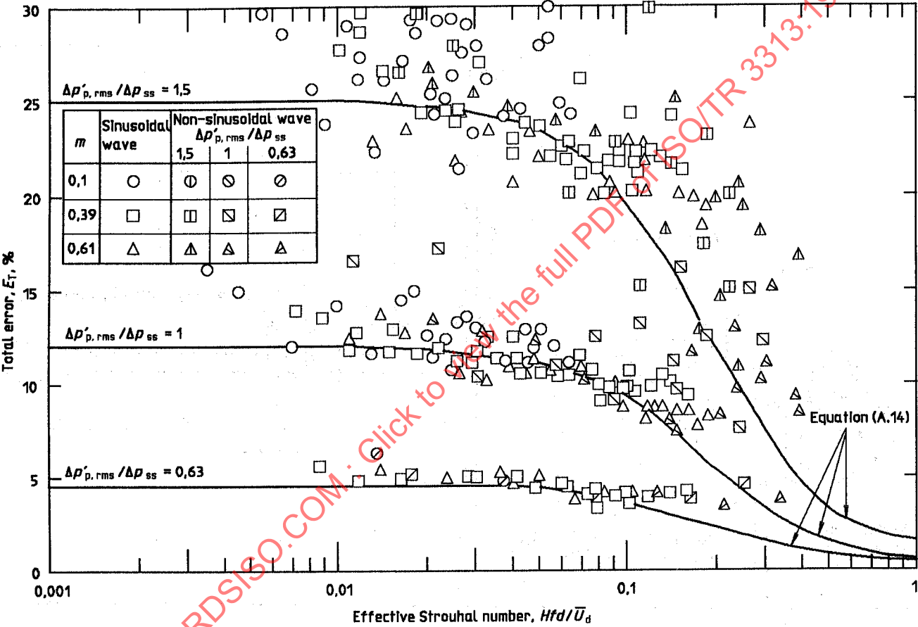
Figure A.2 — Curve of the metering error, E_T , as a function of the effective Strouhal number, Hfd/\bar{U}_d
