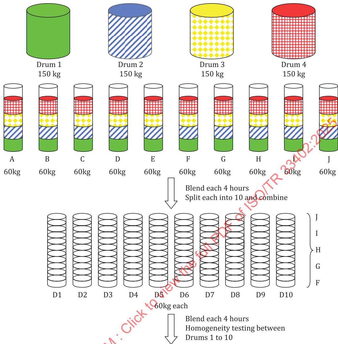
Figure B.1 — Flow diagram of splitting and blending
