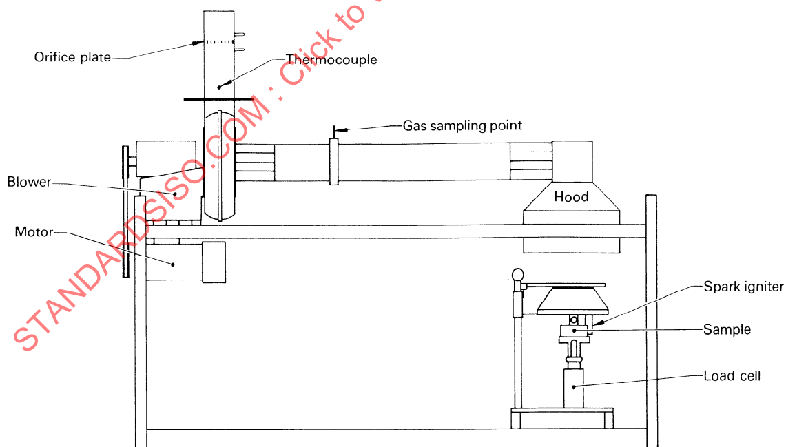
Figure A.3 — ISO heat release test
