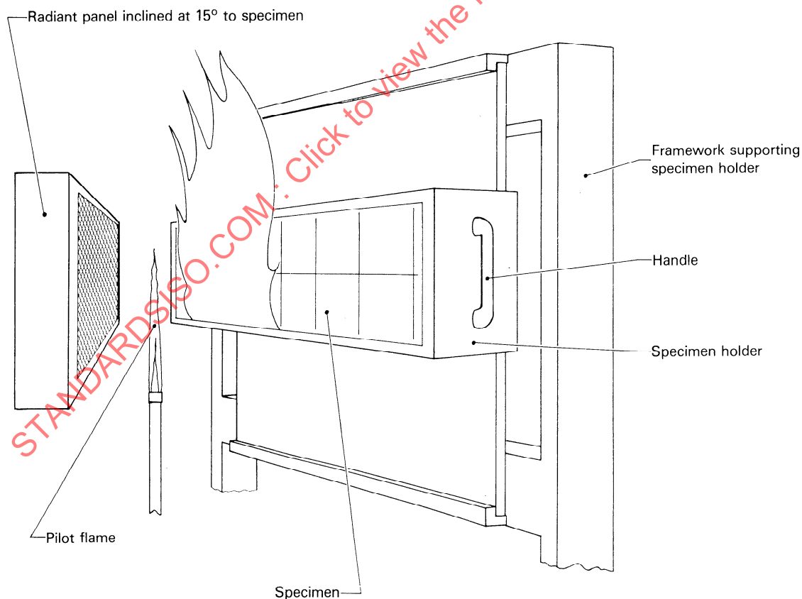
Figure A.2 — Apparatus for surface spread of flame test.
