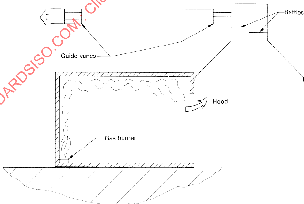
Figure A.6 — ISO room test
