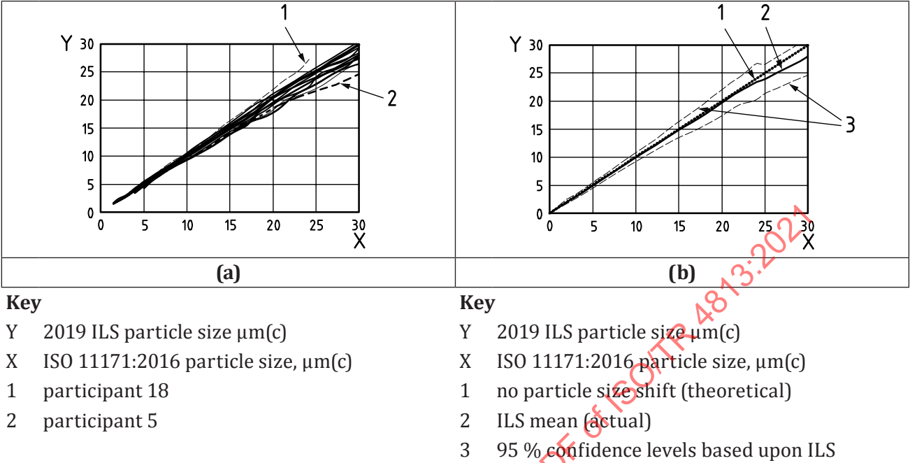
Figure 3 — Graphical summary of 2016 versus 2019 particle sizes for ILS APC
