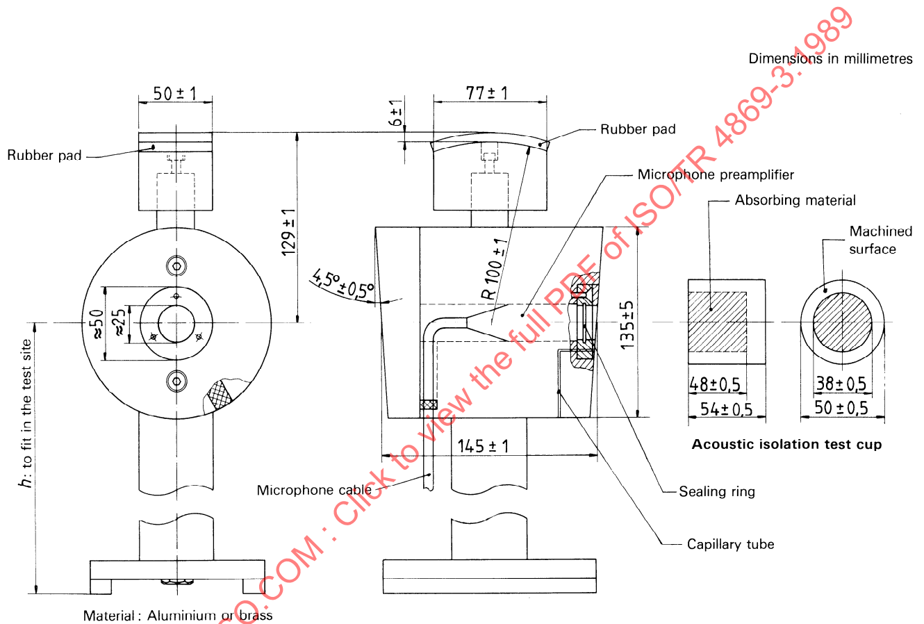
Figure 1 — Example of an acoustic test fixture
