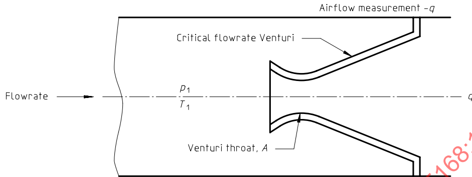
Figure C.5 — Flowrate through a sonic nozzle
