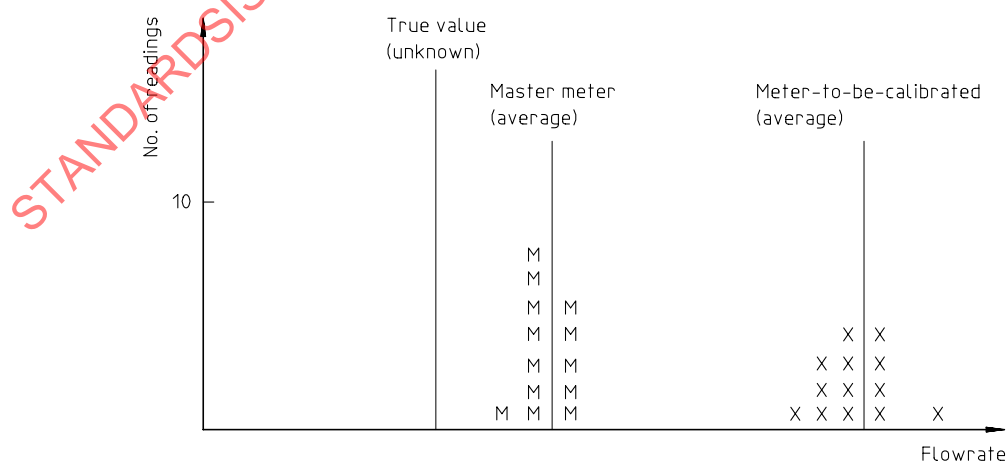
Figure 9 — Calibration should compensate for test meter systematic error
