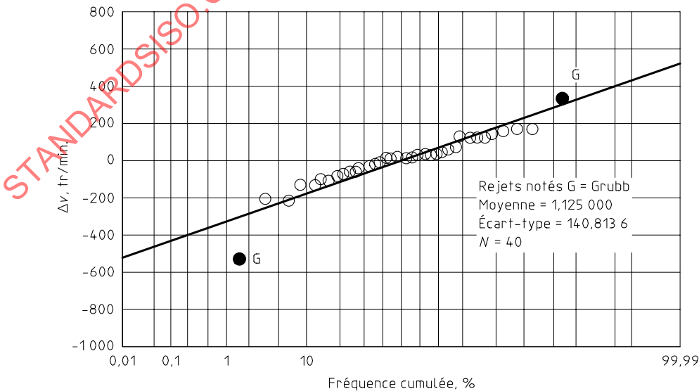
Figure B.2 — Results of outlier tests
