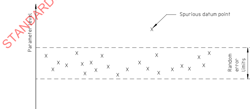
Figure B.1 — Outlier outside the range of acceptable data
