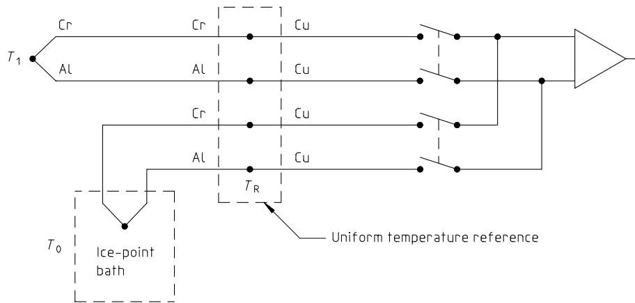
Figure C.4 — Typical thermocouple channel
