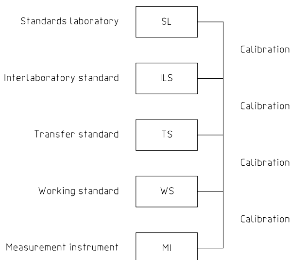
Figure C.3 — Temperature measurement calibration hierarchy
