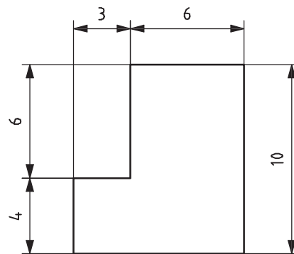
Figure F.2 — L-shaped building
