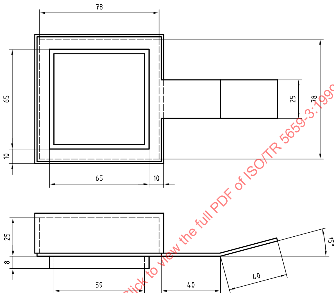
Figure 2 — Specimen holder
