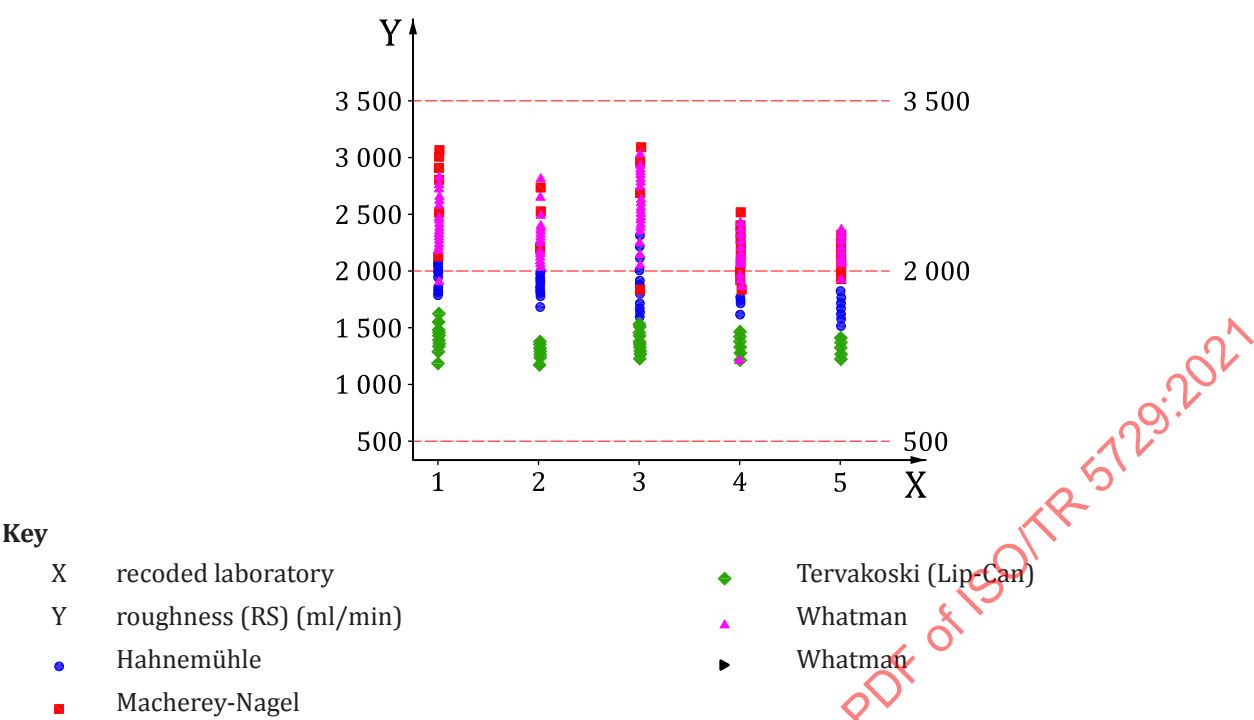
Figure 3 — Scatterplot of Roughness (RS) (ml/min) vs Recoded Laboratory
