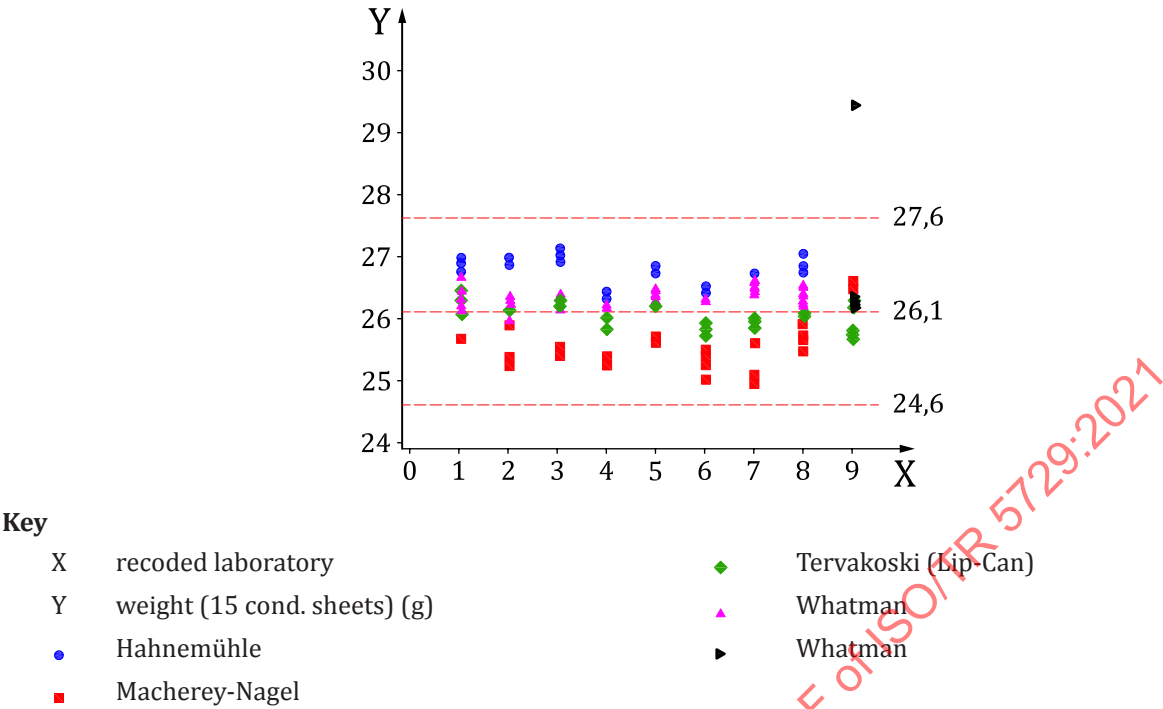
Figure 1 — Scatterplot of Weight (15 Cond. Sheets) (g) vs. Recoded Laboratory
