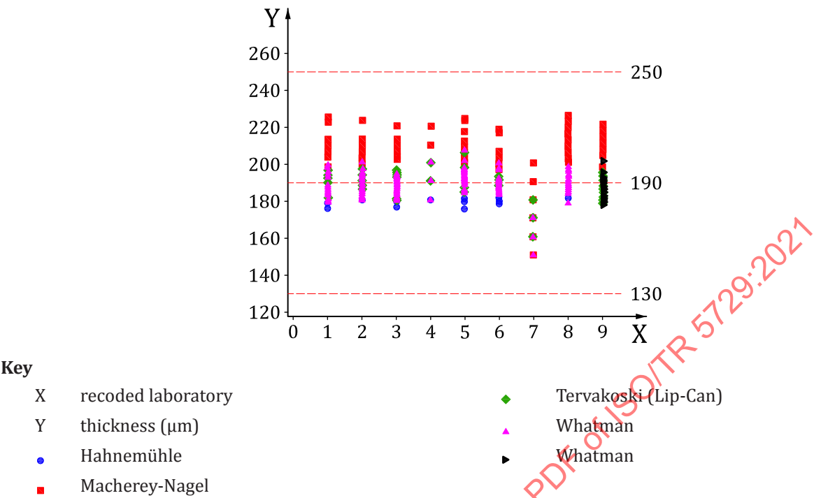
Figure 5 — Scatterplot of Thickness (µm) vs Recoded Laboratory
