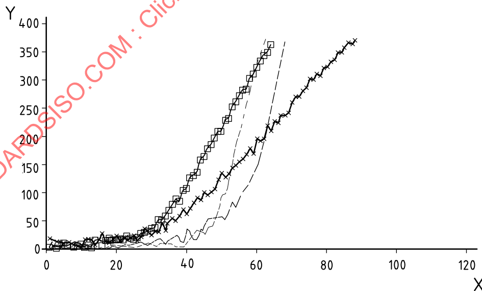
Figure 6 — Loading curves for commercially-available filters tested per ISO 4548-12, when conductivity was not maintained near 1 500 pS/m during the test.
