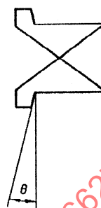
Figure 2 — Expander seating tab angle
