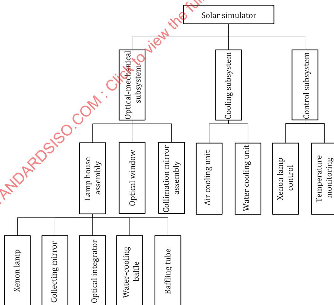
Figure 11 — Composition chart of solar simulator system
