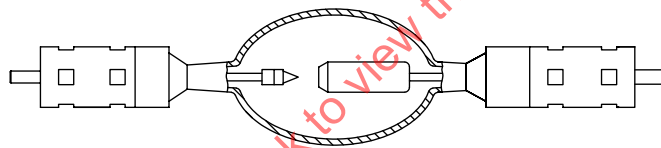
Figure 14 — Short arc xenon lamp
