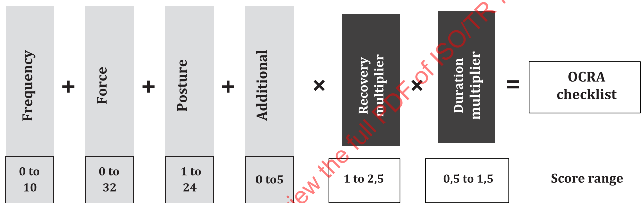
Figure B.1 — OCRA checklist: final score calculation procedure
