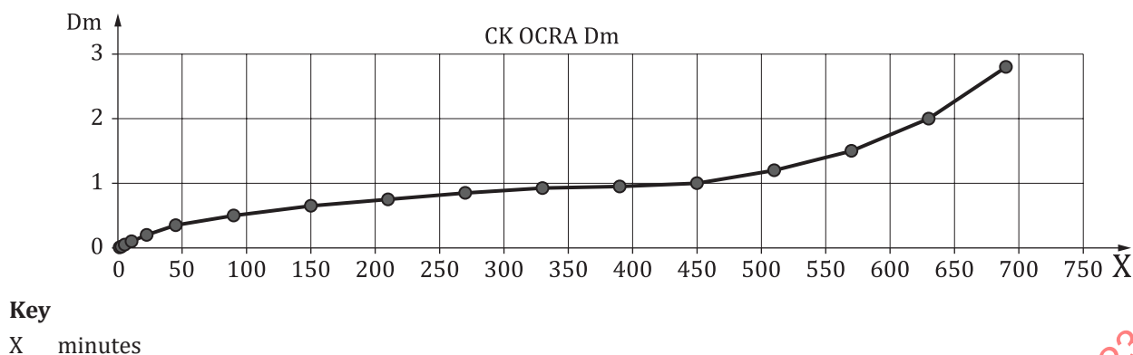
Figure B.2 — Duration multipliers as a function of the duration of repetitive tasks in the shift in the OCRA checklist method
