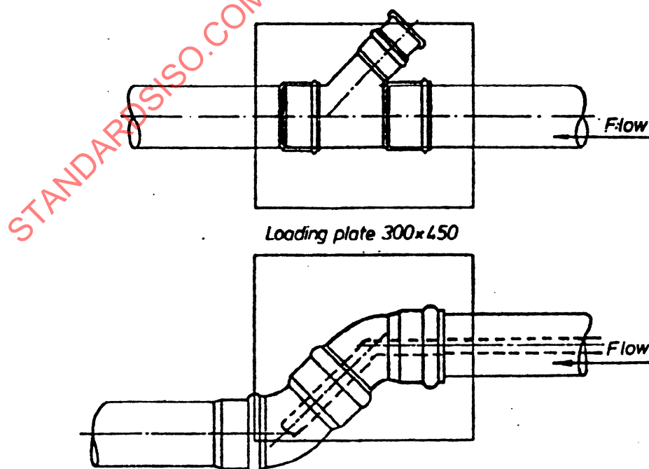
Figure 4. Example of positioning of a fitting under the pressure plate
