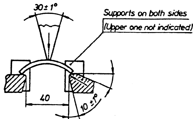
Figure 7. Positioning of a sample
