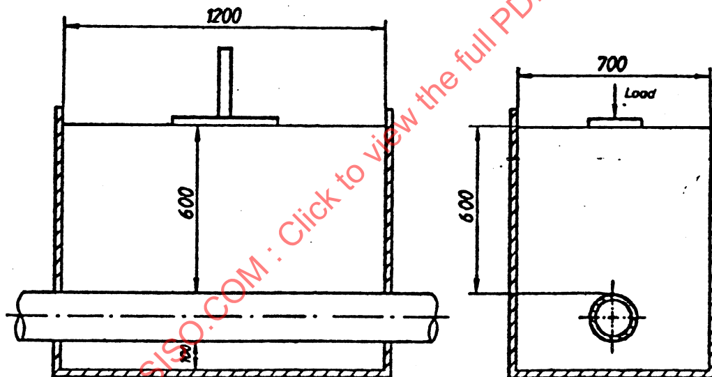
Figure 2. The dimensions of the box
