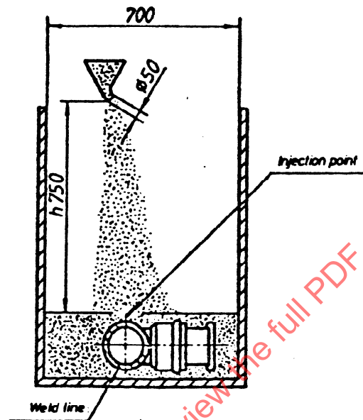
Figure 5. Example of the filling procedure
