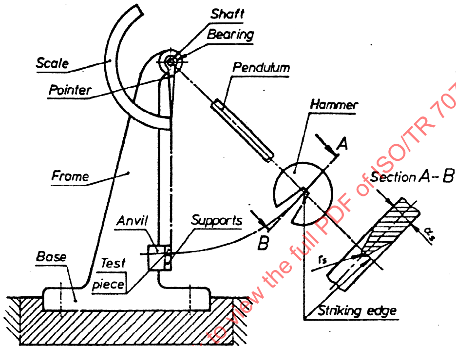
Figure 6. Pendulum impact apparatus
