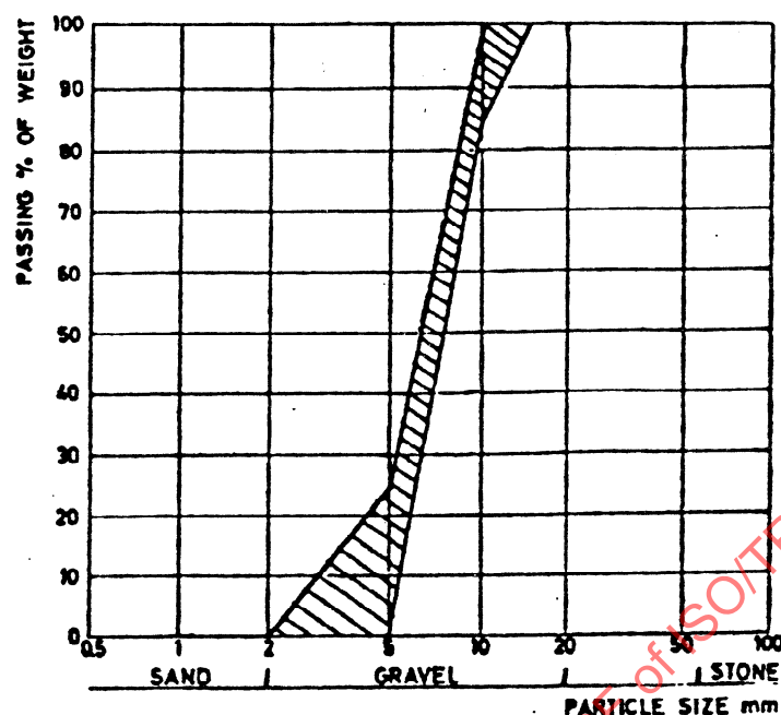
Figure 3. Gradation range of the filling material for BLT-test
