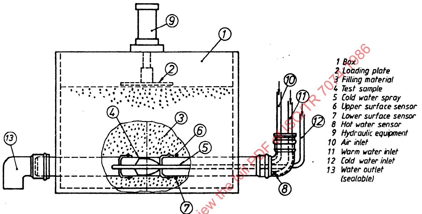
Figure 1. The BLT apparatus
