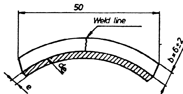
Figure 9. Dimensions of standard curved small testbars.
