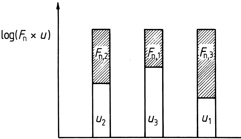
Figure 5 — Test programme B
