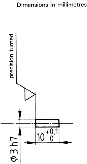
Figure 1 — Test specimen — Pin
