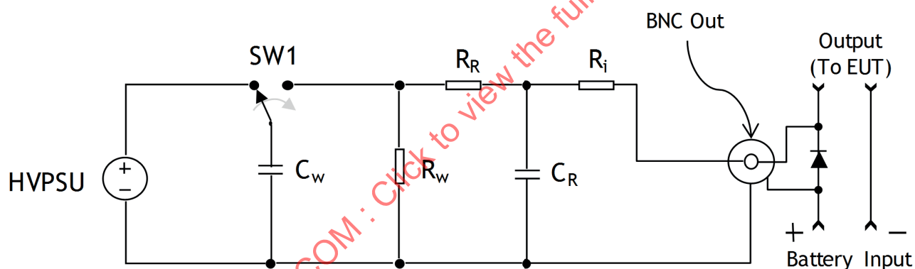
Figure 5 — Decoupling network with diode
