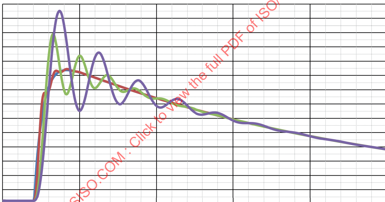
Figure 6 — Coupling network example pulse 2a
