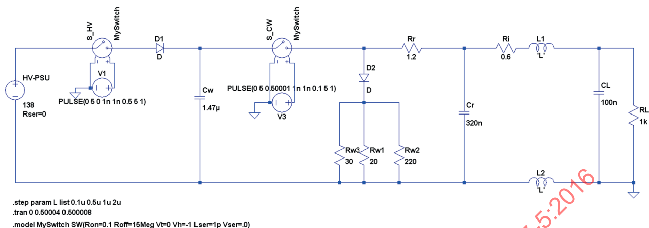
Figure 6 — Coupling network example pulse 2a
