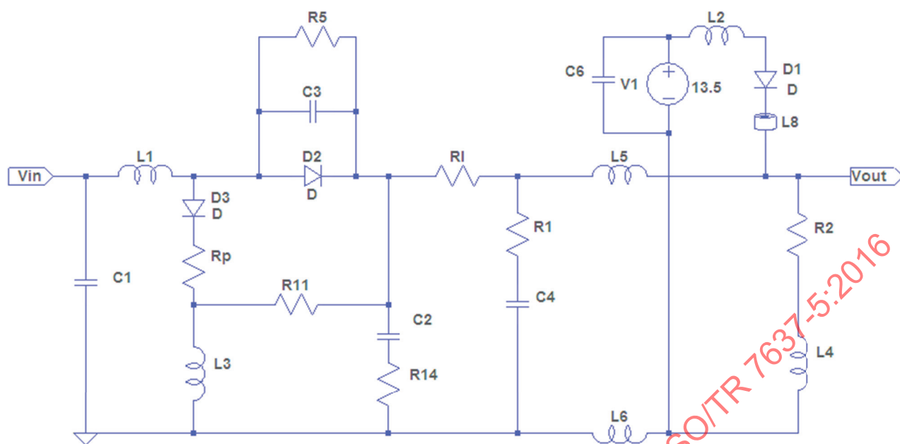
Figure 4 — Decoupling network with chokes
