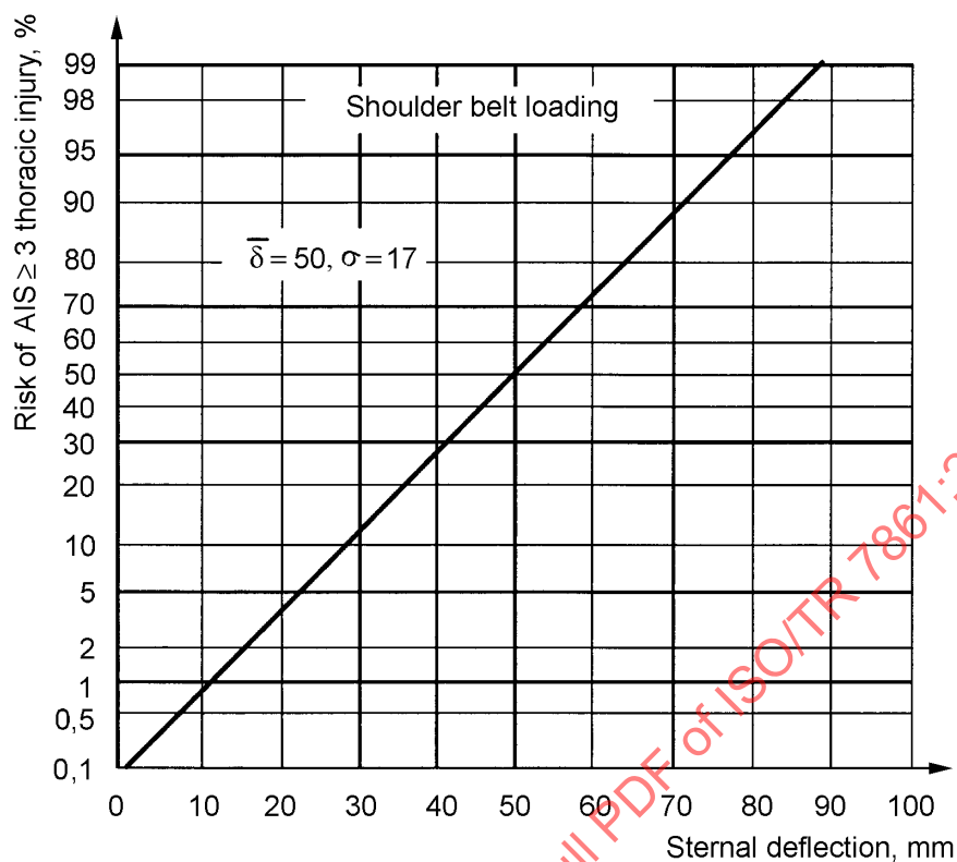
Figure A.7 — Risk of AIS \geq 3 thoracic injury due to shoulder belt loading as function of peak Hybrid III sternal deflection
