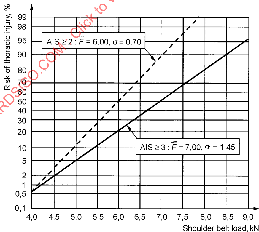
Figure A.8 — Risk of AIS \geq 2 and \geq 3 thoracic injury as function of peak shoulder belt load
