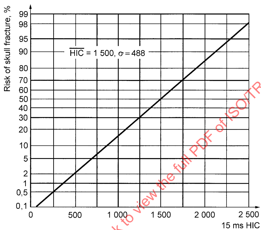
Figure A.1 — Risk of AIS ≥ 2 skull fracture as function of max. 15 ms HIC
