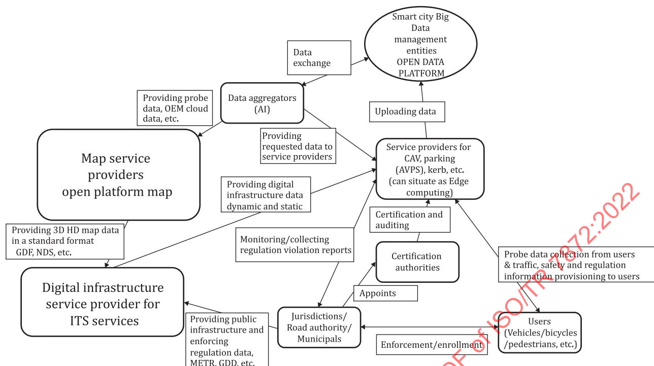
Figure 2 — Role model and functional model of digital infrastructure servicer
