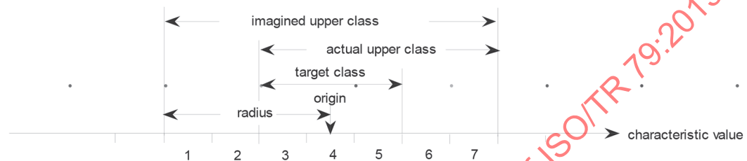
Figure 8 — Diagram of similarity on different types of characteristics, Case D: categorical or ordinal characteristic
