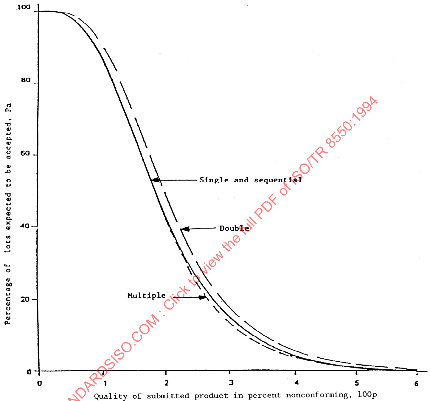
Figure 6 Comparison of operating characteristic curves for single, double, multiple and sequential sampling plans (code letter L, AQL 0,65%)
