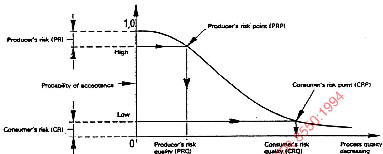
Figure 1 - Operating characteristic curve defined by producer's risk (PR) and consumer's risk (CR)
