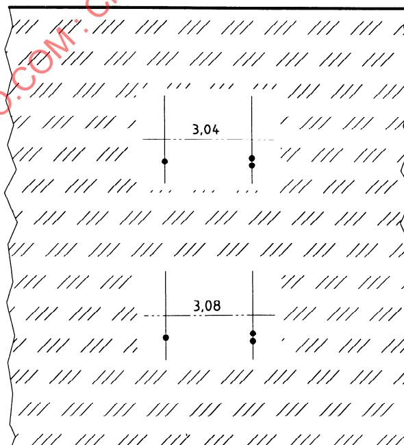
Figure D.1 — Optical limit gauge for verifying the diameter of the applanation circle (in this case set for a value of 3,06 mm)
