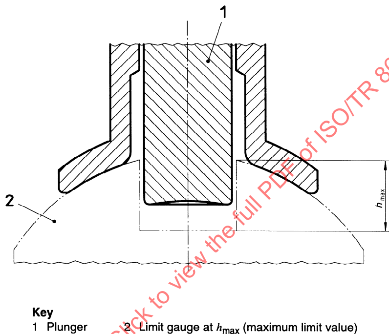
Figure C.11— Verification of extension of plunger below footplate
