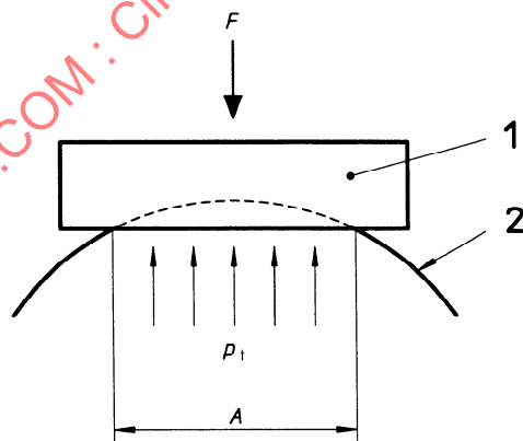
1 Pressure body
