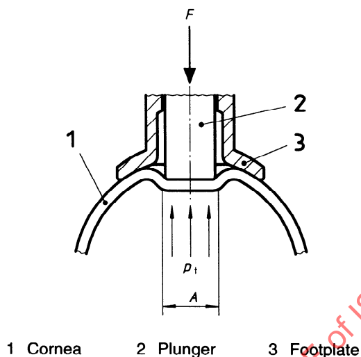
Figure A.2 — Principle of impression tonometry
