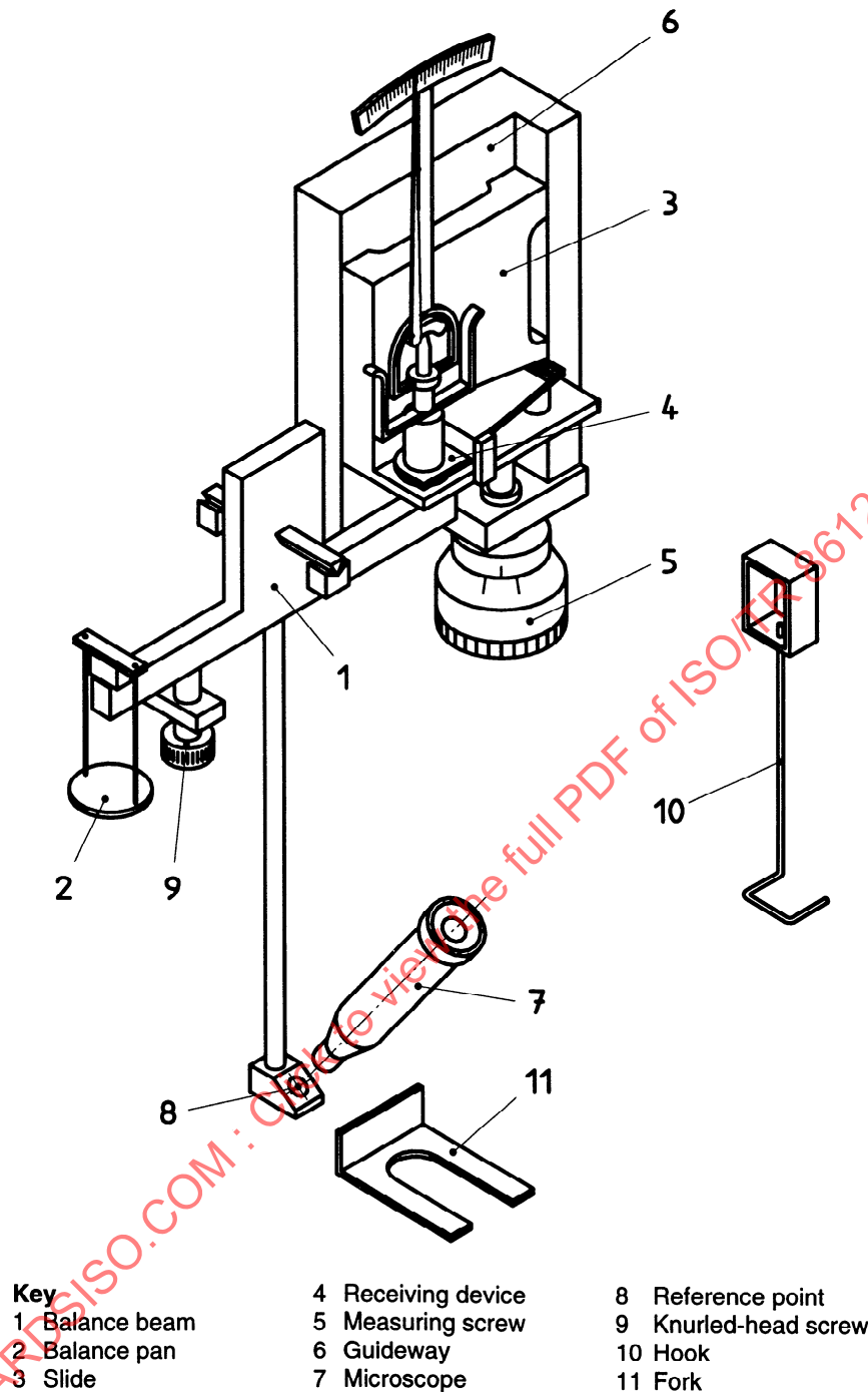
Figure C.1 — Arrangement for verifying effective weight of the plunger loaded by lever-pointer system, displacement of the plunger and mass of tonometer (without handle)
