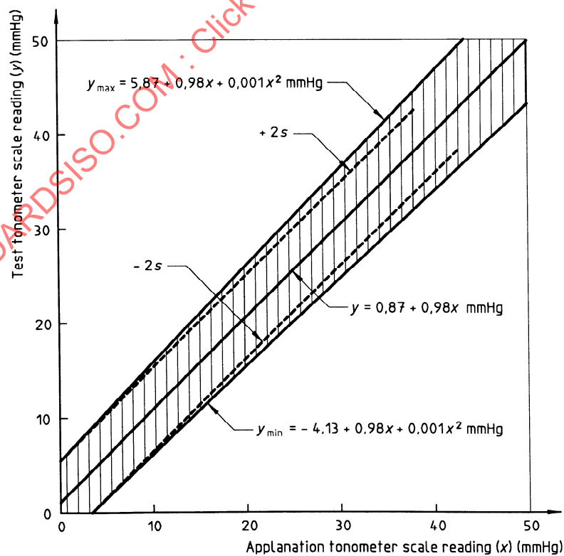
Figure B.2 — Example of a regression curve and the tolerance area for y values [15], [16]
