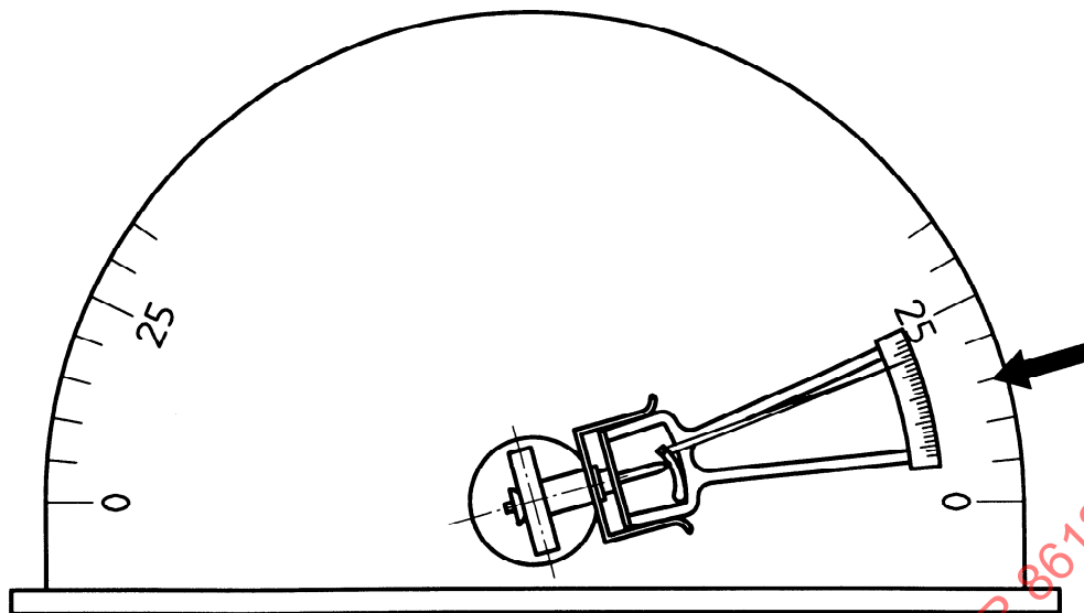
Figure C.2 — Measuring apparatus for testing friction between plunger and plunger sleeve
