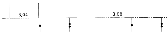
Figure D.2 — Verification of tolerance limits for the diameter of the applanation circle (in this case having a value of 3,06 mm)
