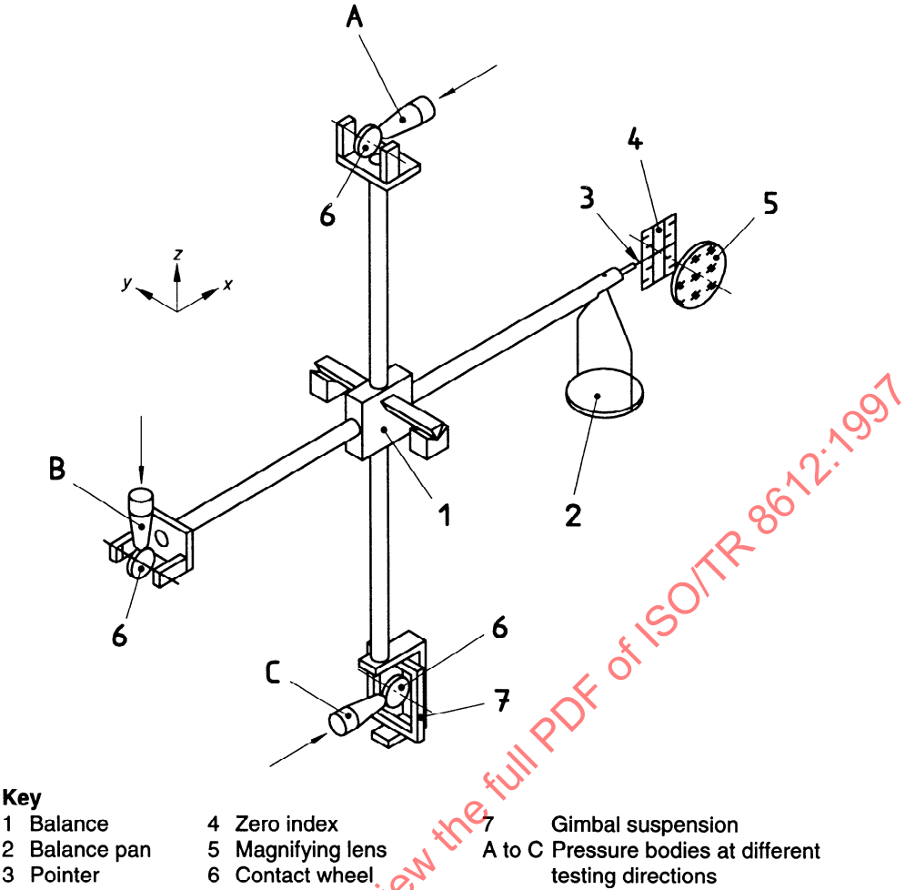
Figure D.3 — Arrangement for verifying the measuring force
