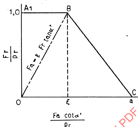
FIGURE 4-5 — Dynamic equivalent radial load for radial contact groove ball bearings
