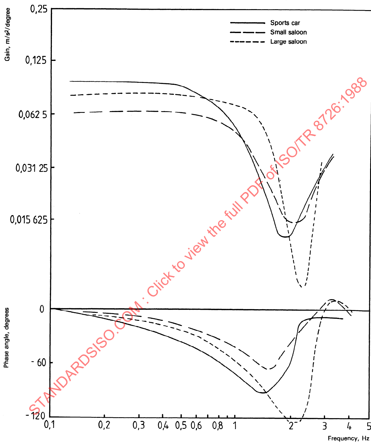
Figure 5 — Typical lateral acceleration responses to steering-wheel input at 80 km/h
